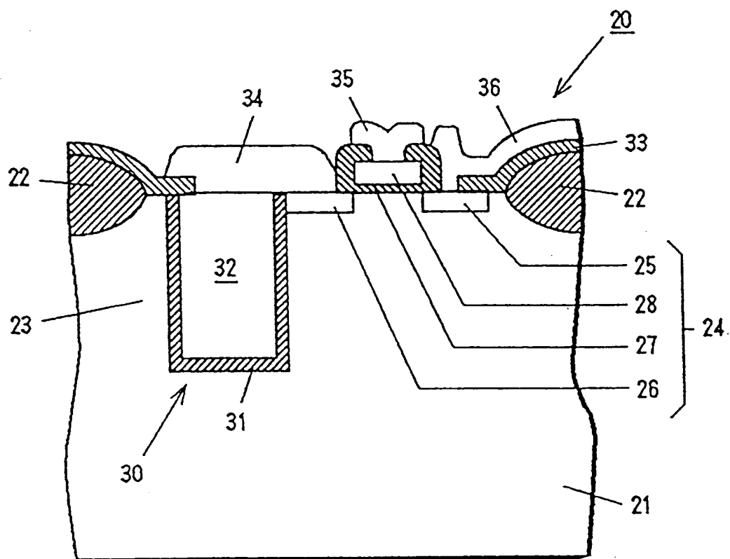
FIG. 18 PRIOR ART
