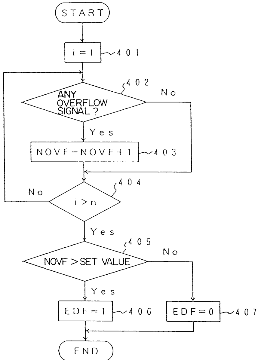
FLOWCHART ILLUSTRATING OPERATION OF STATE MONITORING PART
