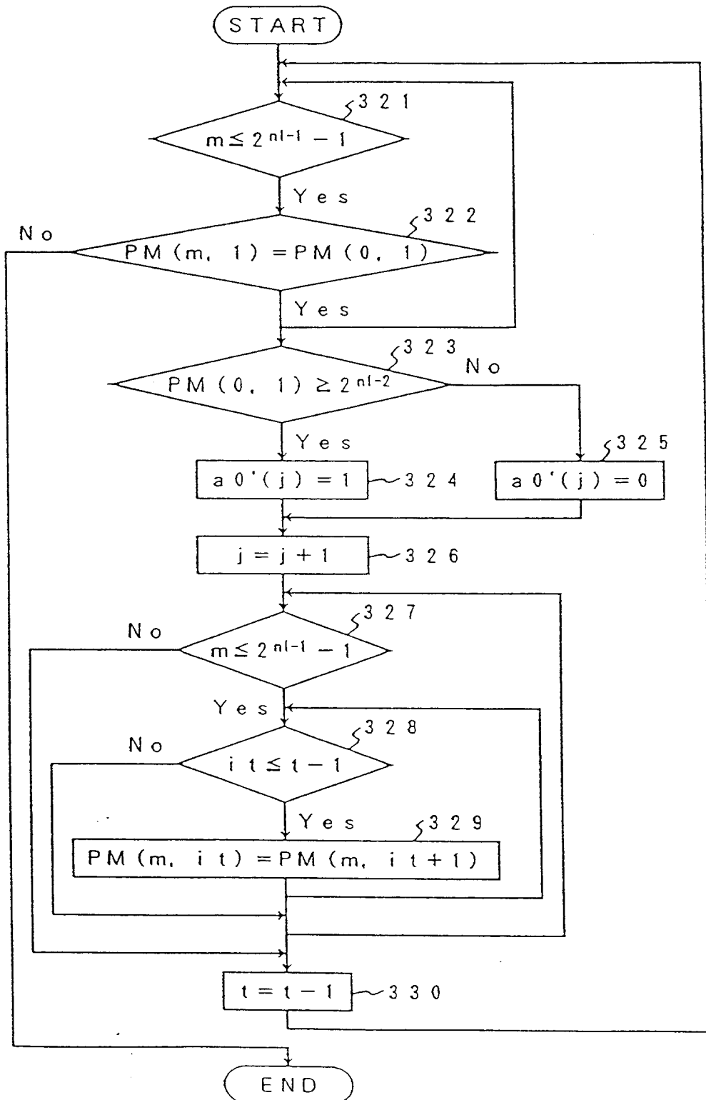
FLOWCHART ILLUSTRATING OPERATION OF STEP 2
