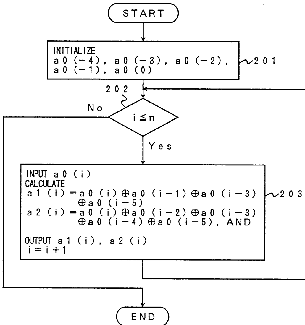
FLOWCHART ILLUSTRATING OPERATION OF ERROR CORRECTING/ENCODING PART
