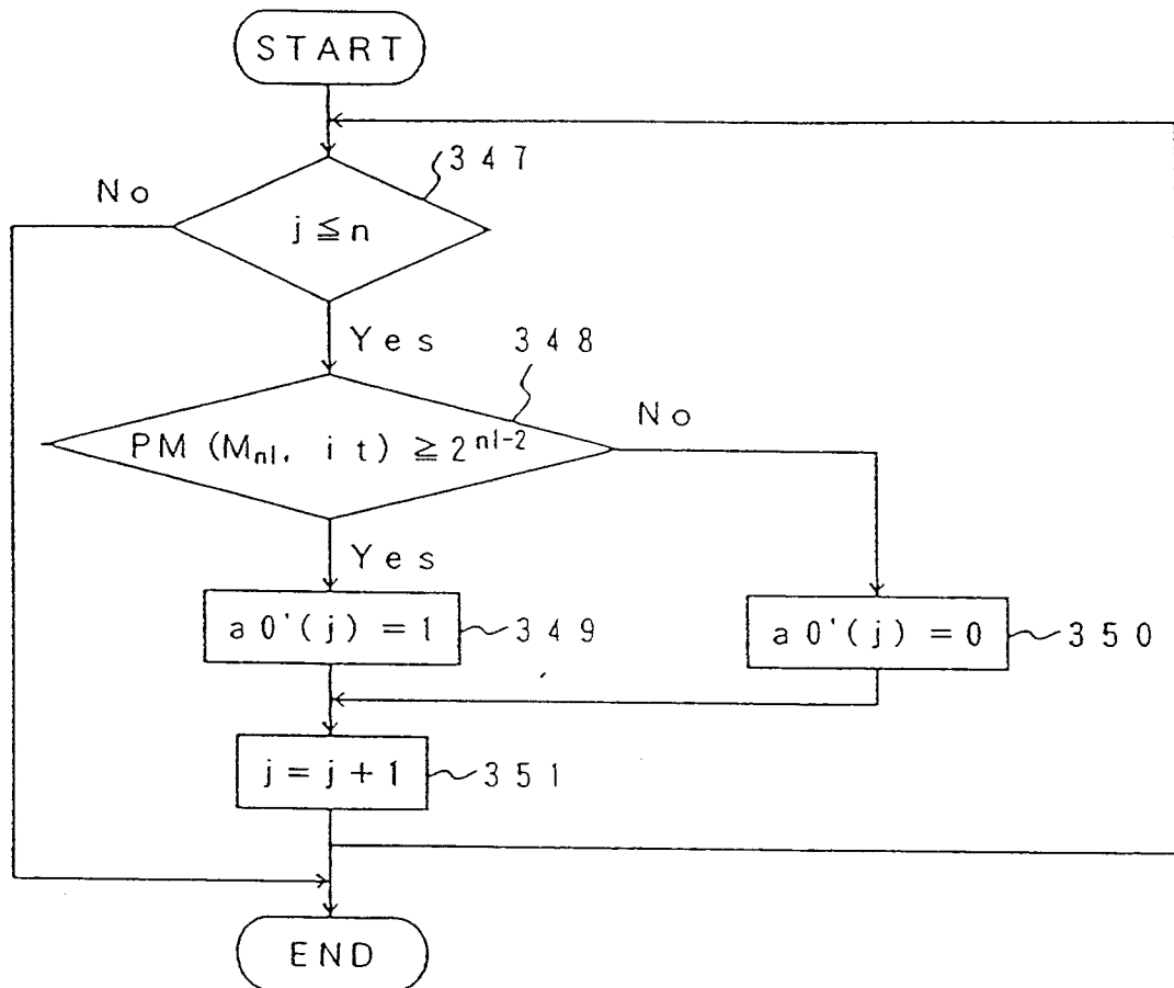
FLOWCHART ILLUSTRATING OPERATION OF STEP 4
