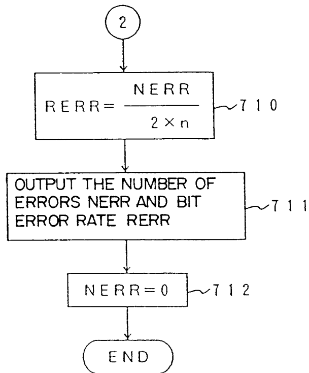
FLOWCHART ILLUSTRATING OPERATION OF THE COMPARATOR PART
