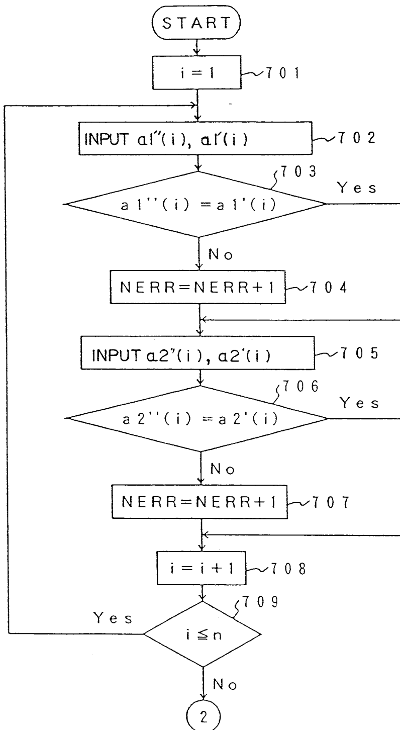
FLOWCHART ILLUSTRATING OPERATION OF THE COMPARATOR PART
