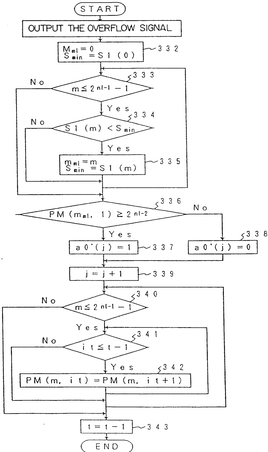
FLOWCHART ILLUSTRATING OPERATION OF STEP 3
