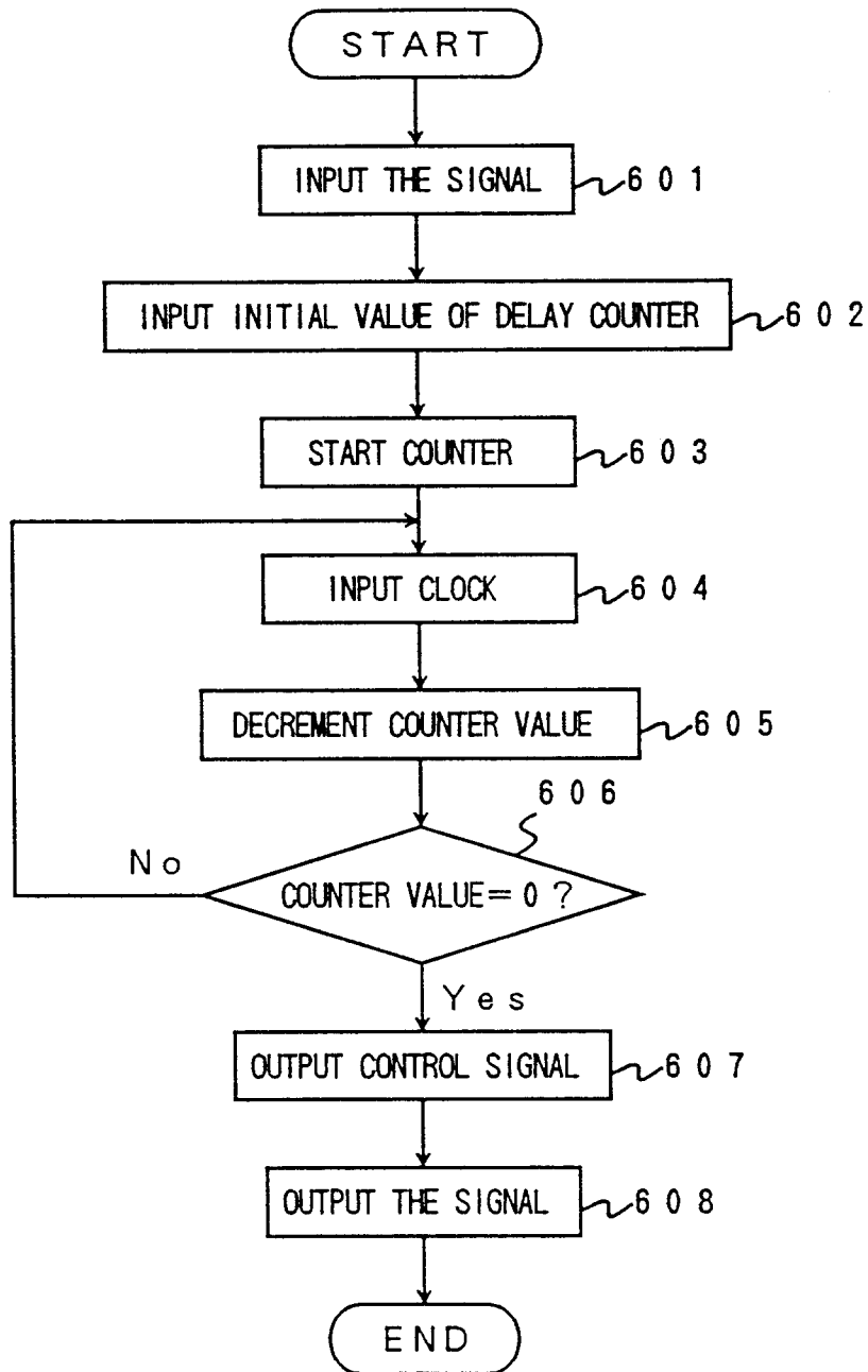
FLOWCHART ILLUSTRATING OPERATION OF THE DELAY PART
