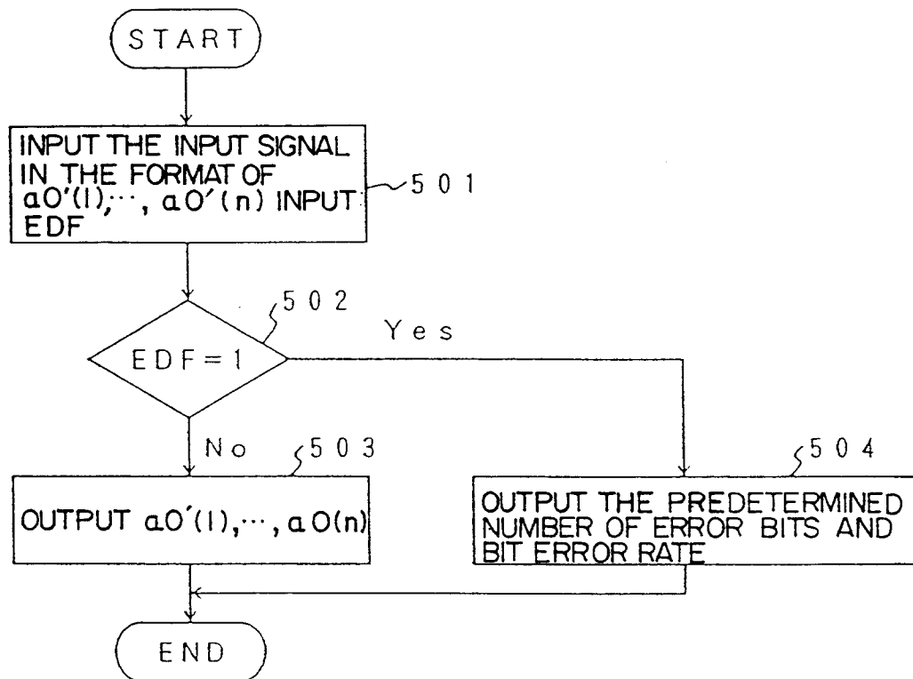
FLOWCHART ILLUSTRATING OPERATION OF SWITCHING PART
