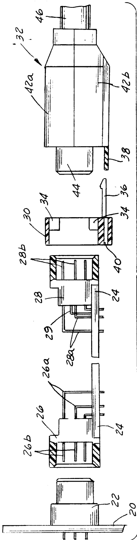
FIG. 1 (PRIOR ART)
