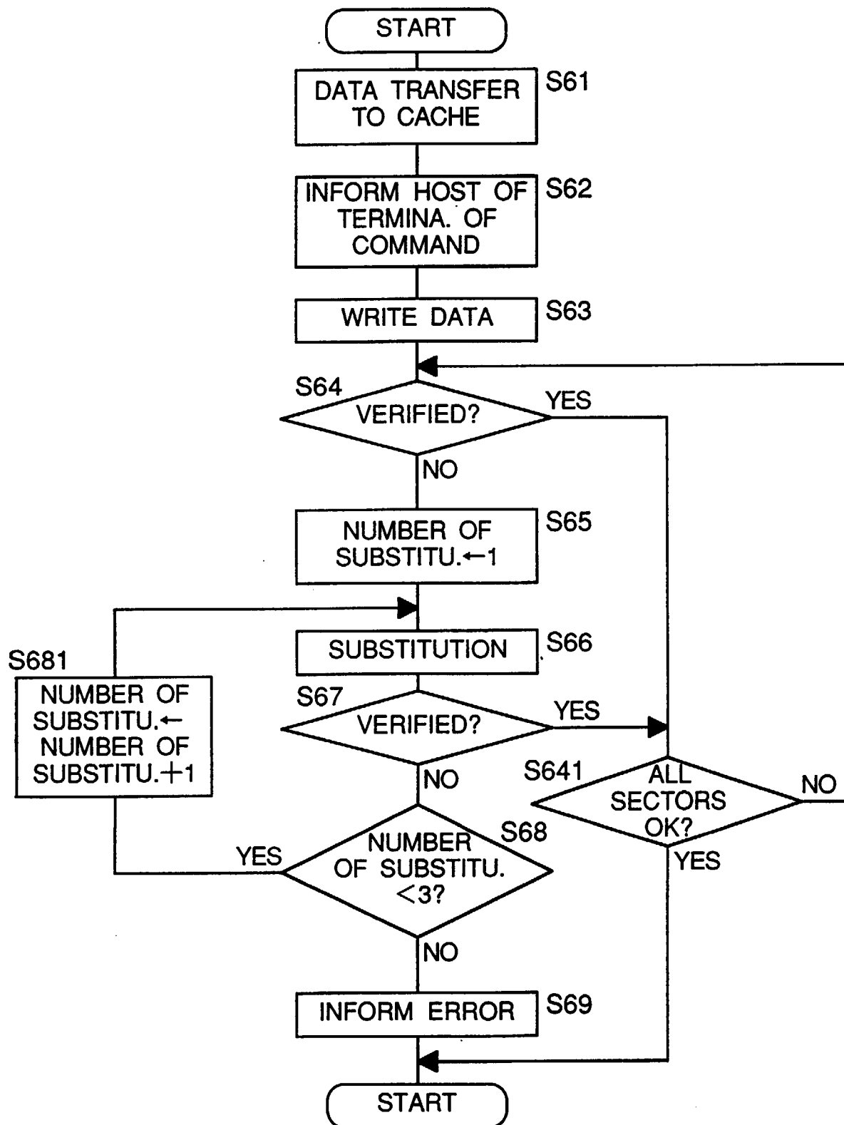
Fig.6 PRIOR ART
