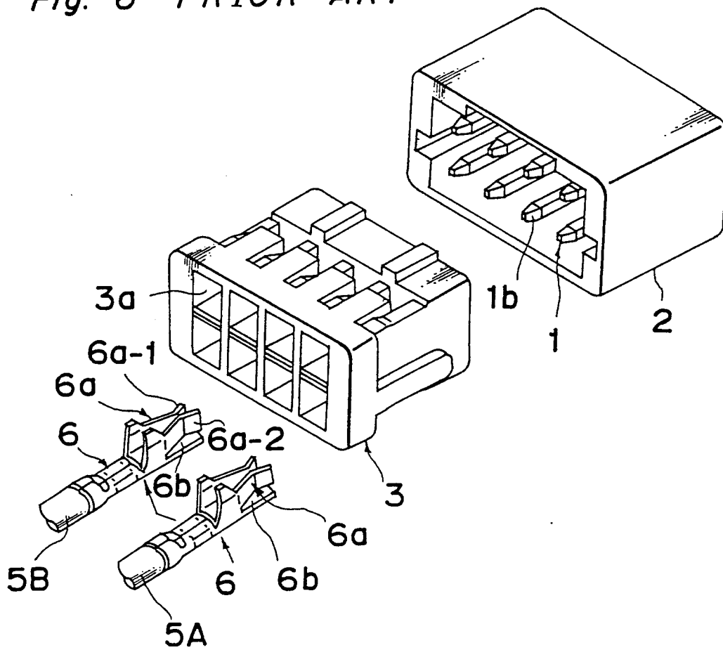
Fig. 6 PRIOR ART
