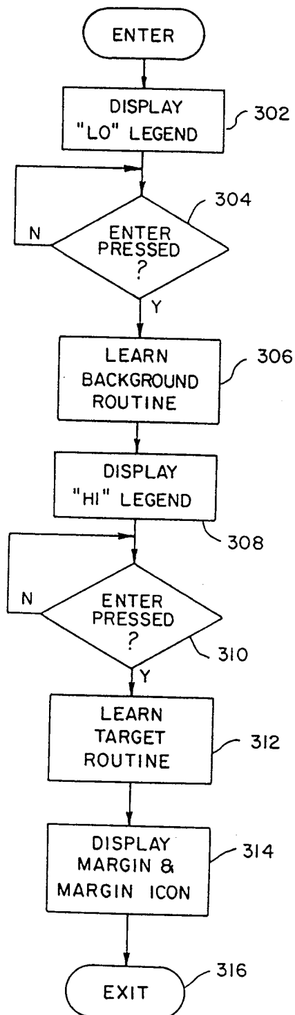
FIG. II LEARN AGS ROUTINE
