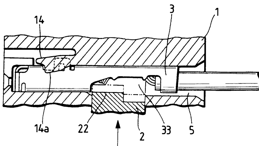
FIG. 8 (RELATED ART)
