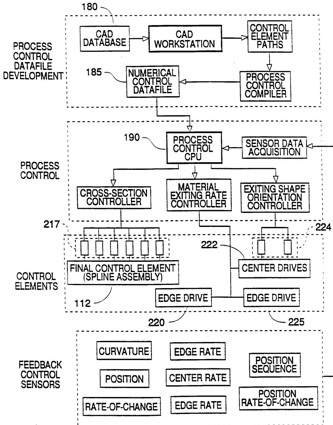
FIG. 11 — SYSTEM BLOCK DIAGRAM
