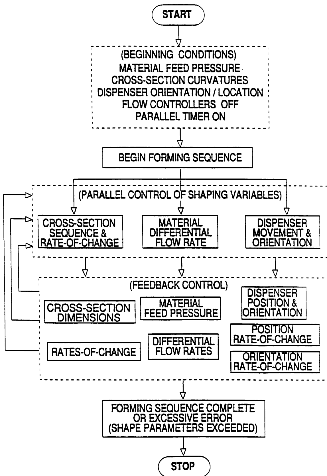
FIG. 14 — PROCESS CONTROL DIAGRAM
