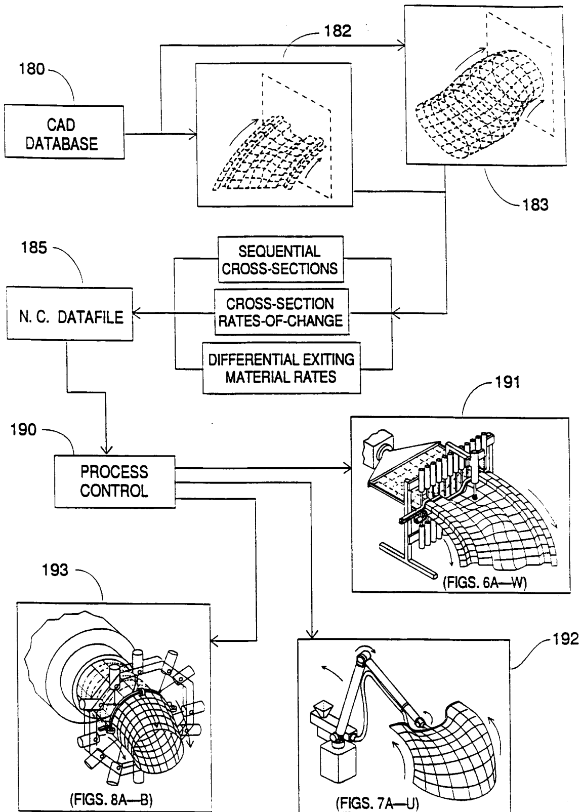
FIG. 5 — PROCESS OVERVIEW
