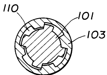
FIG.15 (PRIOR ART)
