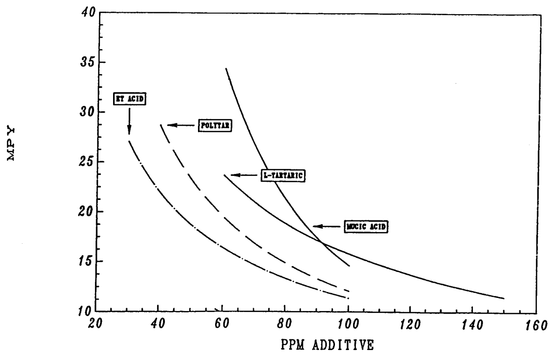
FIGURE 1 CORROSION RATE IN 6XCTW/2X ALK
