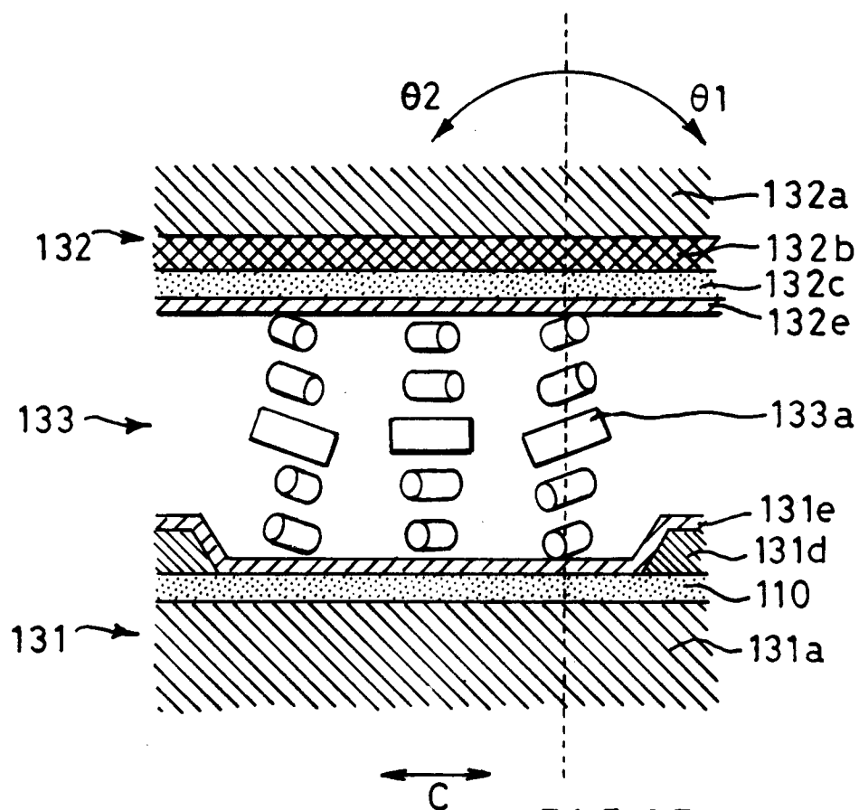
FIG.27. PRIOR ART
