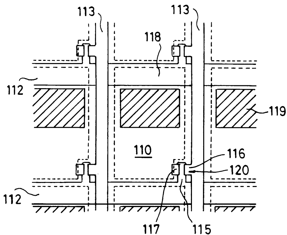
FIG.26. PRIOR ART
