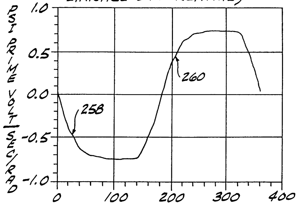
FIG. 5B BACK EMF PROPORTIONAL (FLUX LINKAGE DIFFERENTIAL)
