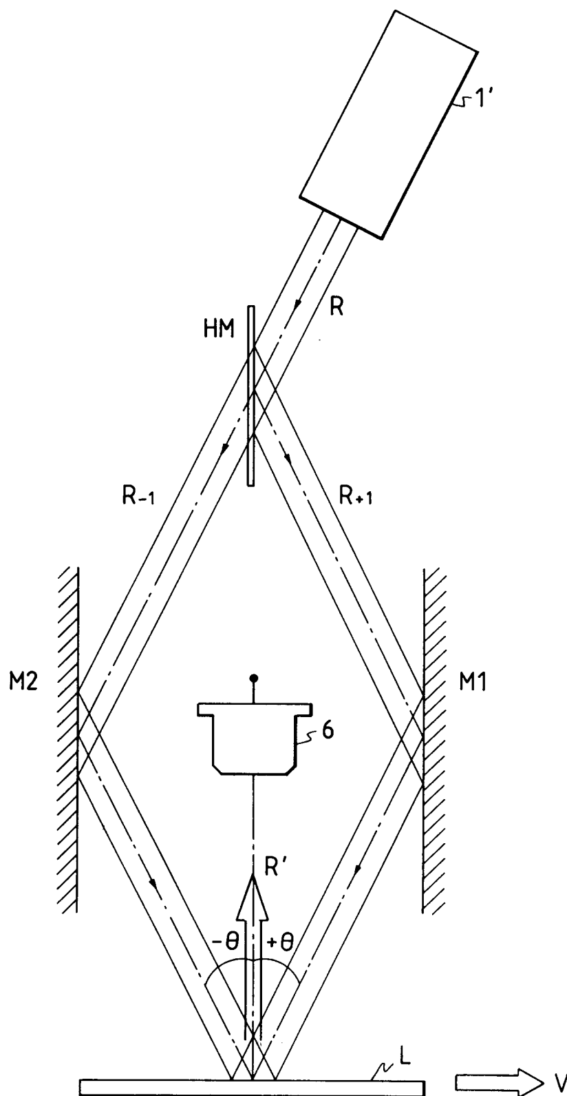
FIG. 1 PRIOR ART
