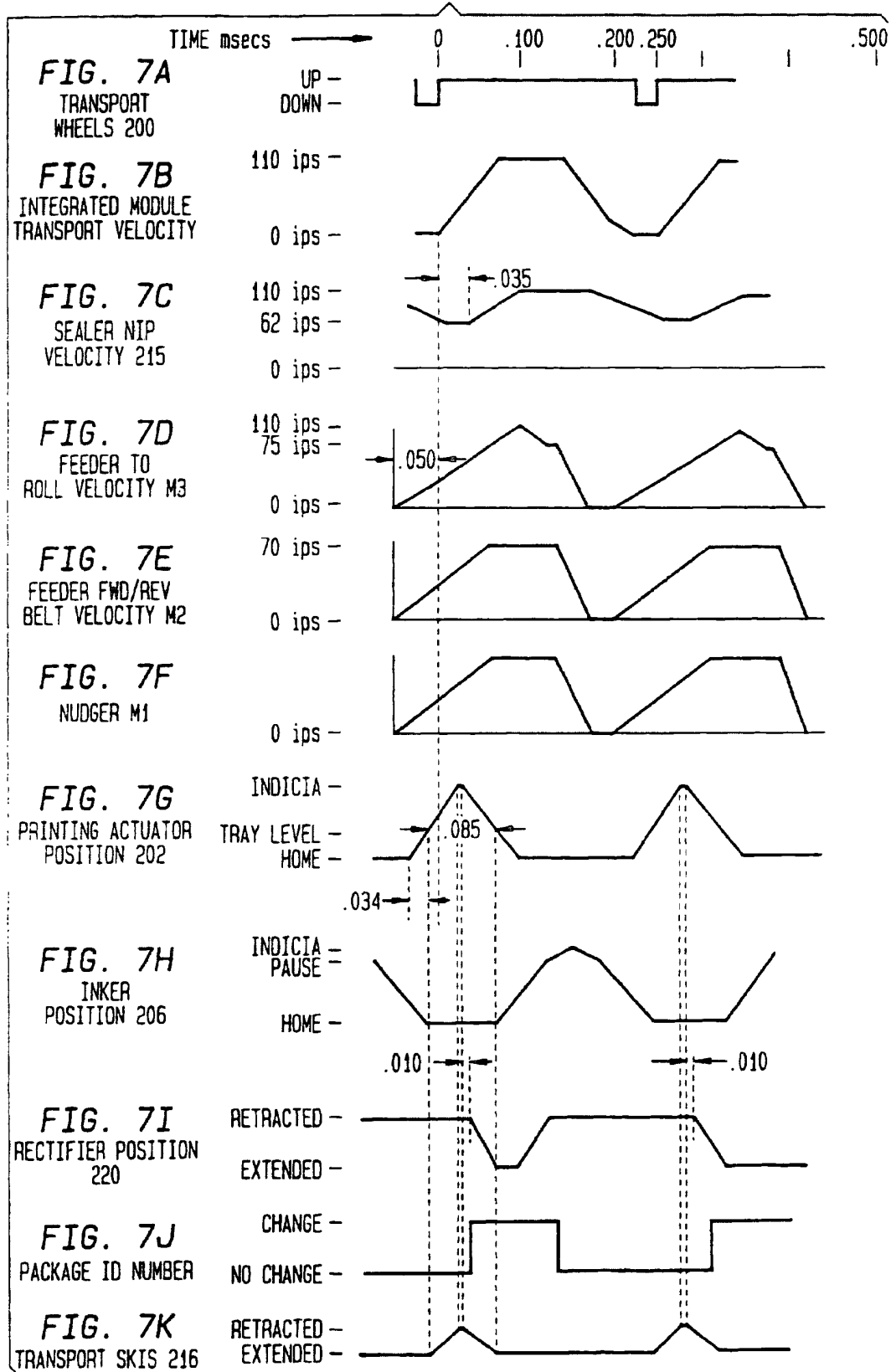
FIG. 7 MODEL TIMING (NON-WEIGH/No 10 ENVELOPE)
