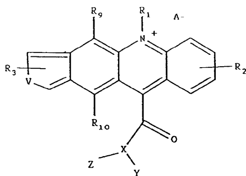
Formula III C
