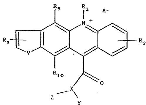
Formula III B
