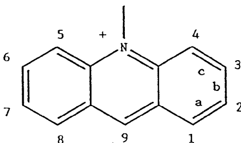
Acridinium nucleus
