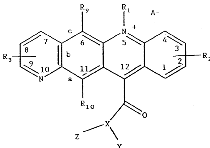
Formula IV D: Pyrido[2,3-b]acridinium compounds
