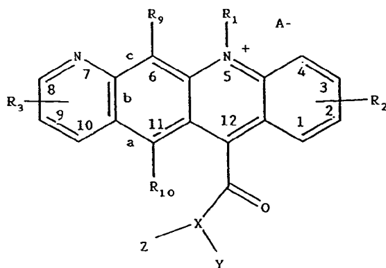
Formula IV A: Pyrido[5,6-b]acridinium compounds
