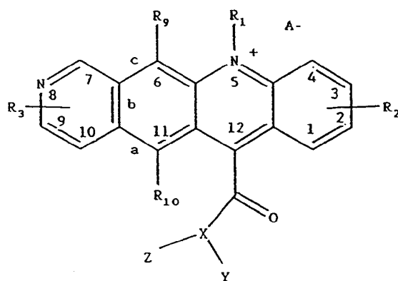
Formula IV B: Pyrido[4,5-b]acridinium compounds
