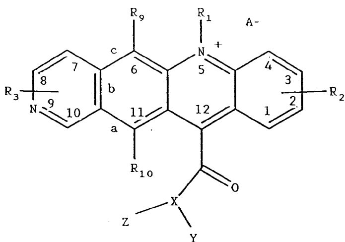
Formula IV C: Pyrido[3,4-b]acridinium compounds
