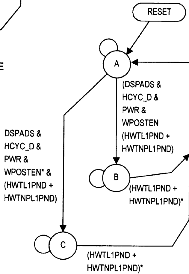
HWL2PND STATE MACHINE
