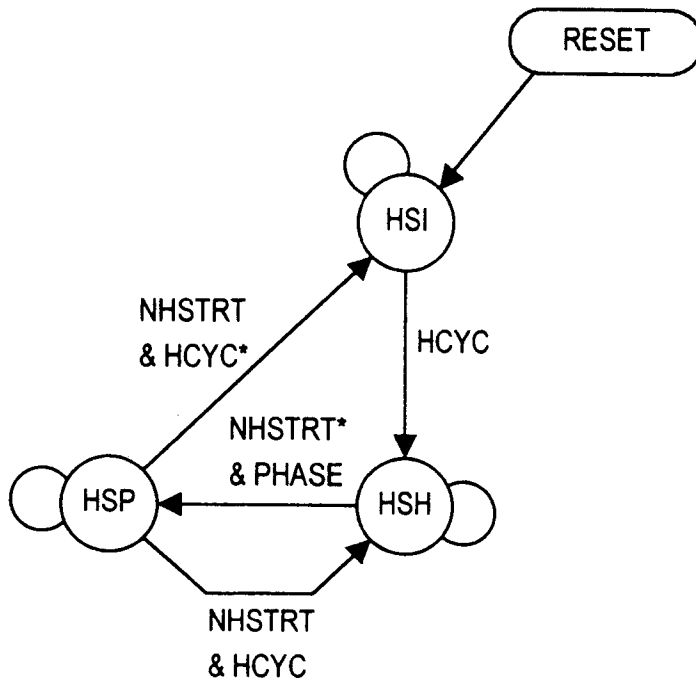
HSYNC STATE MACHINE
