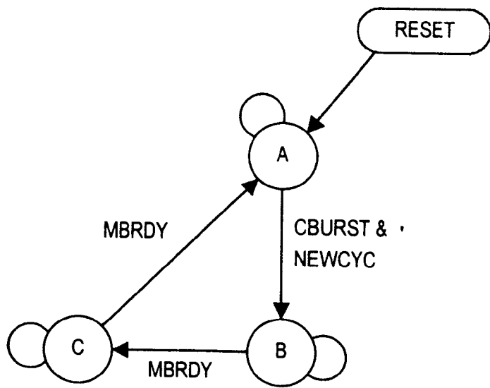
BURST STATE MACHINE
