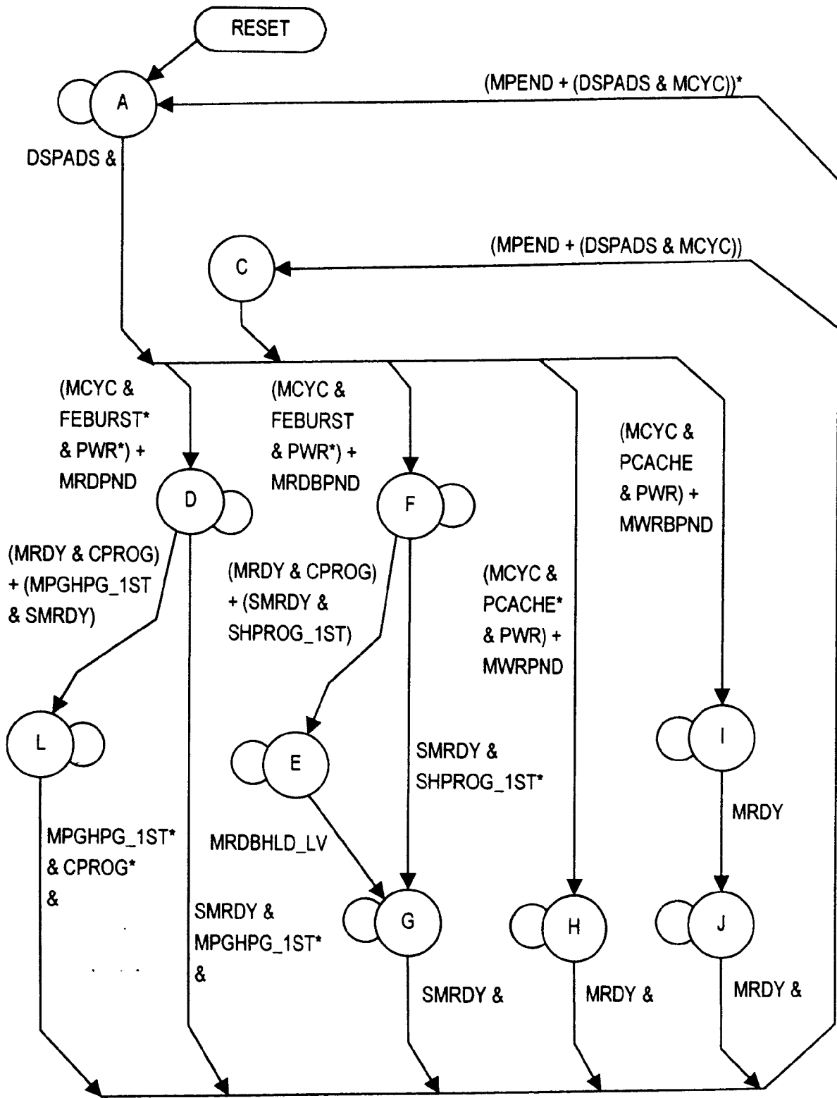
MProg STATE MACHINE
