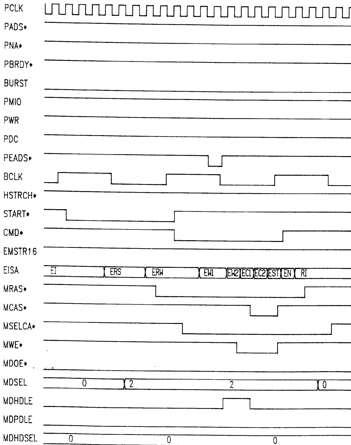
EISA BUS MASTER WRITE CYCLE
