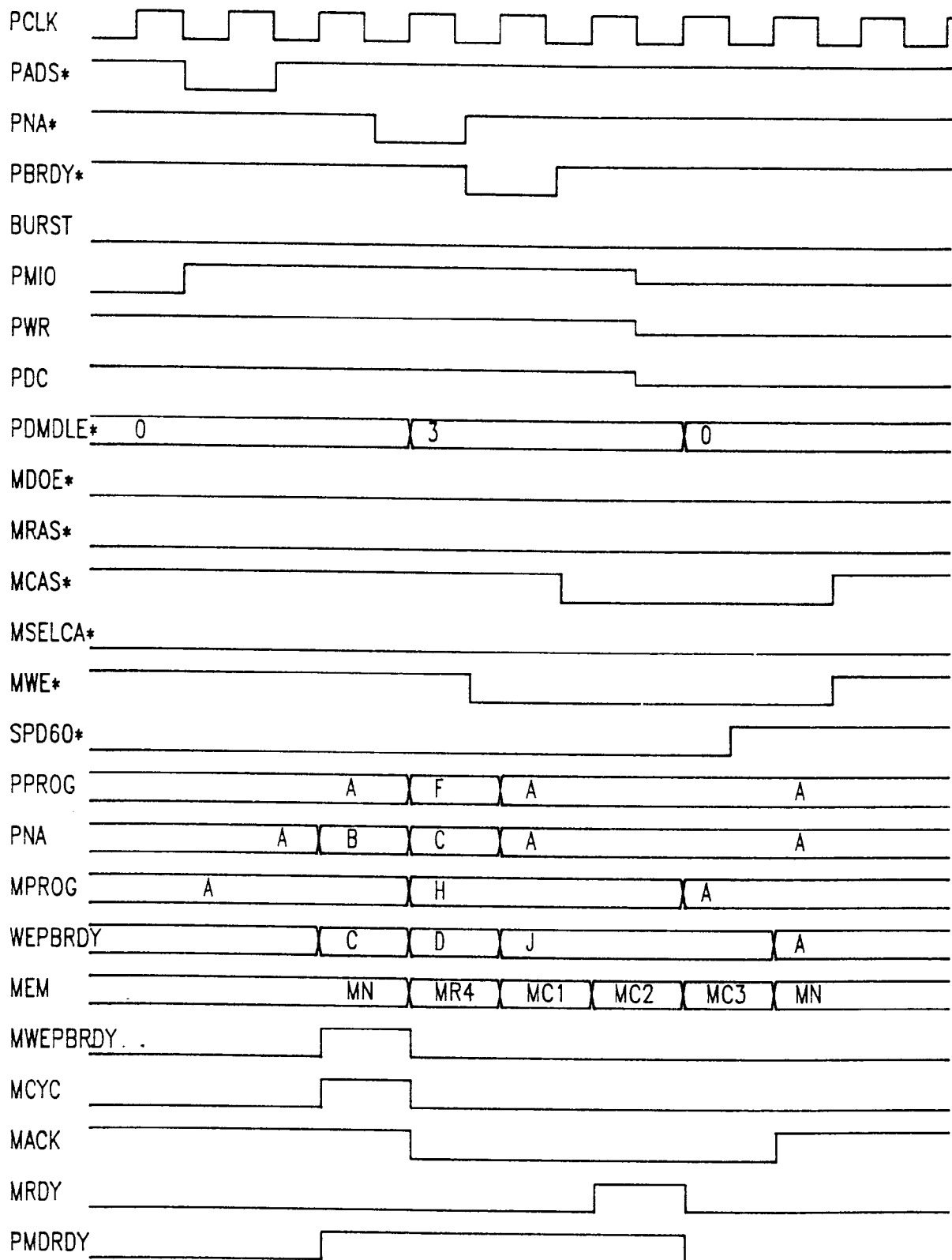
MEMORY WRITE, PAGE HIT, w/60ns MEMORY
