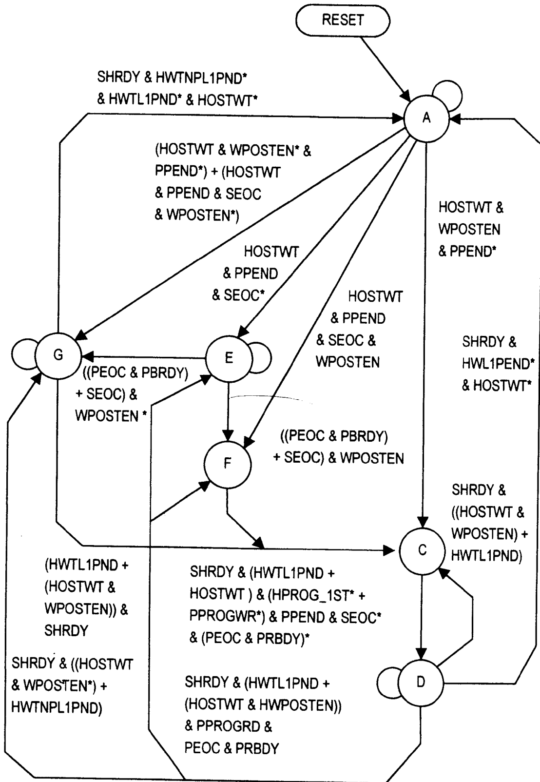
HWT STATE MACHINE
