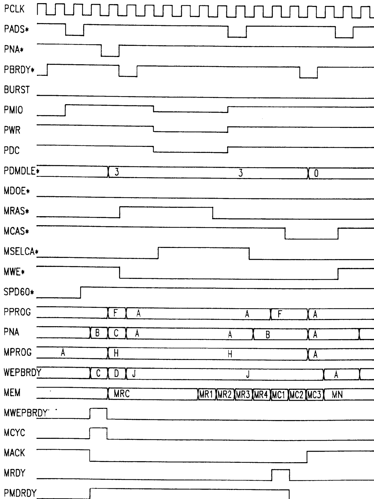
MEMORY WRITE, PAGE MISS, w/80ns MEMORY
