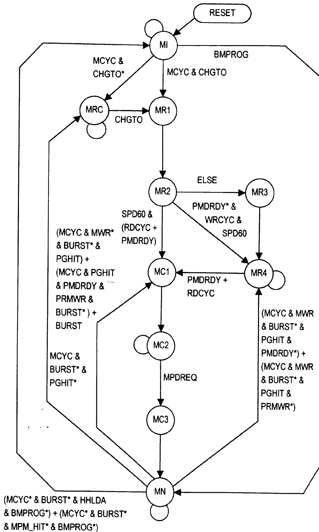
MEM STATE MACHINE
