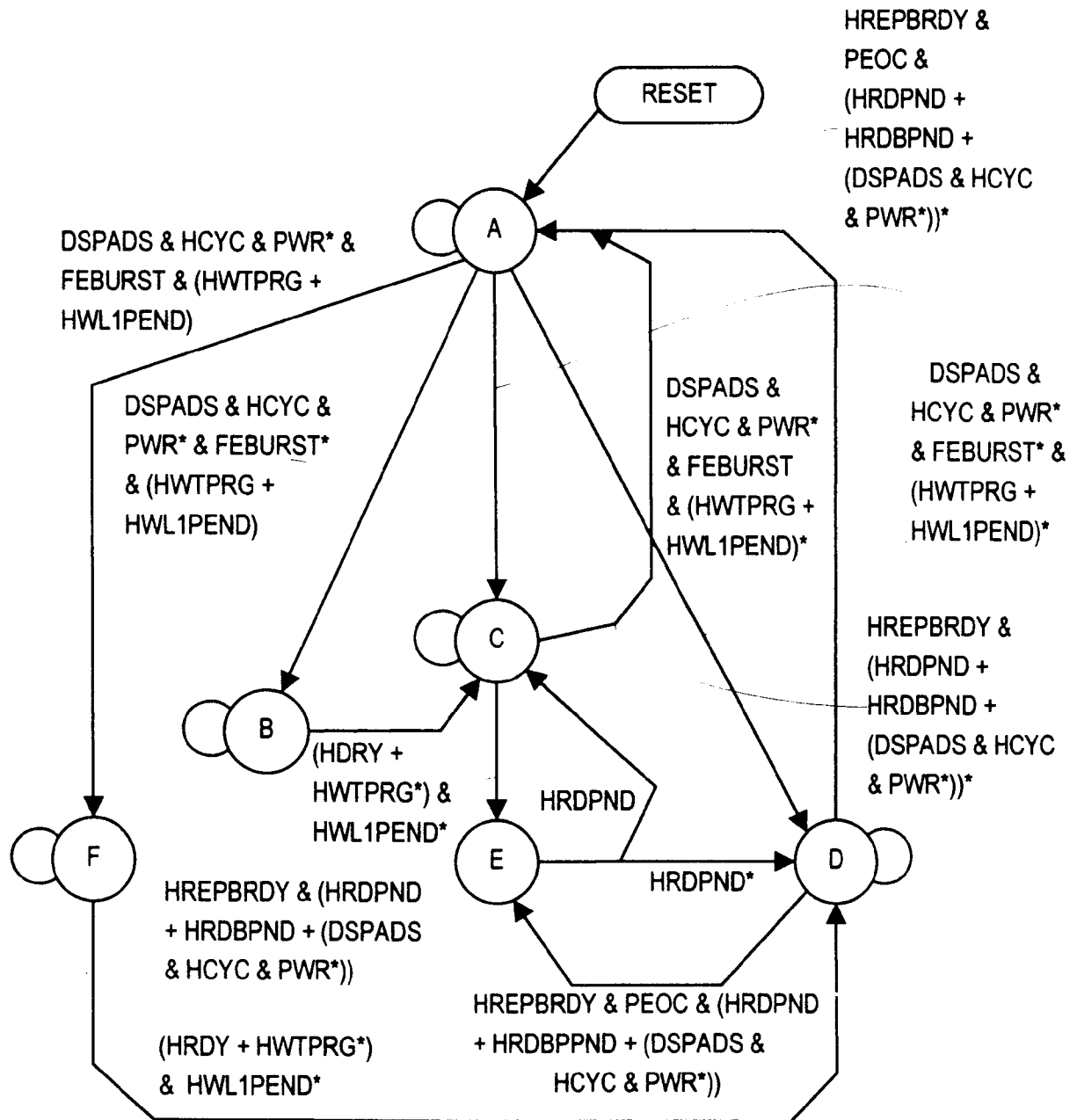
HRD STATE MACHINE
