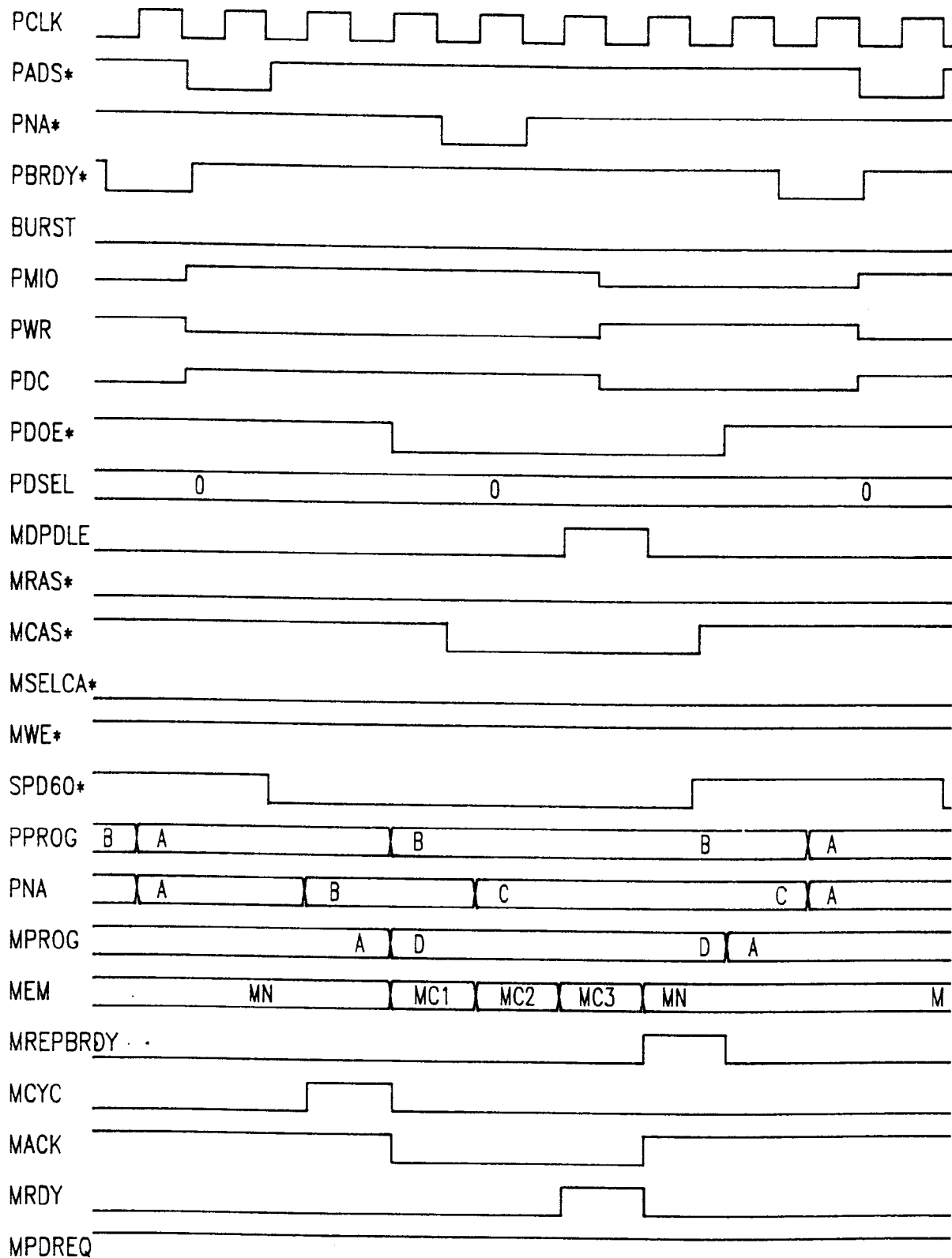
MEMORY READ, PAGE HIT, w/60ns MEMORY
