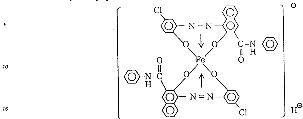
Complex [I]-7
