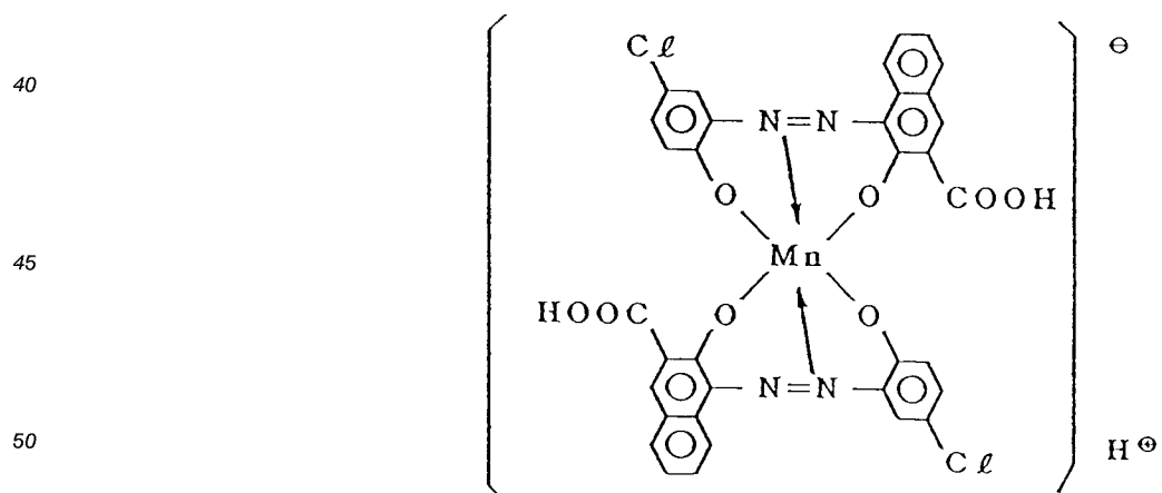
Complex [I]-6
