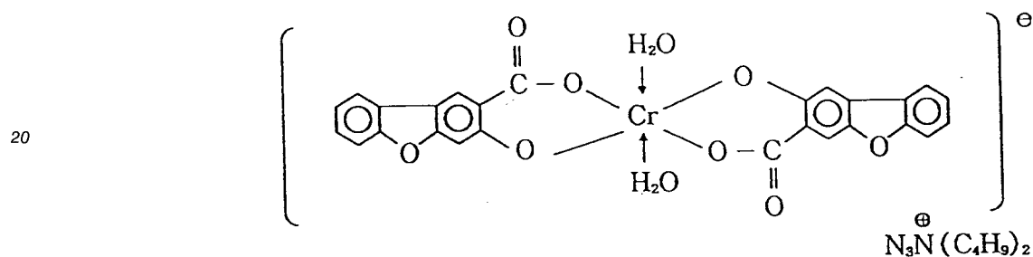
Complex [II]-6
