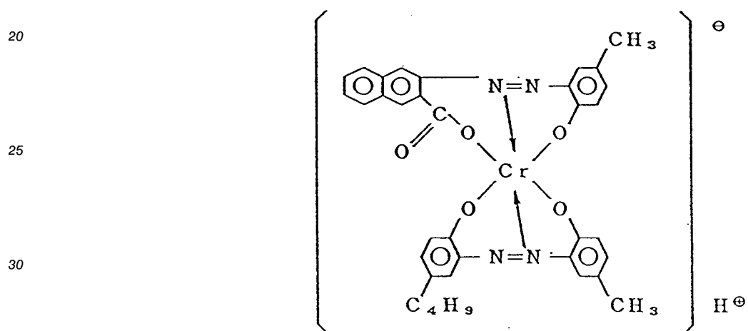
Complex [I]-5
