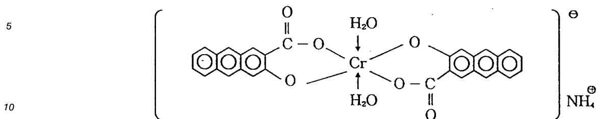
Complex [II]-4
