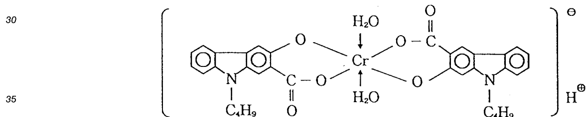
Complex [II]-6
