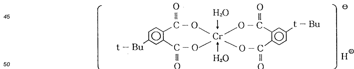
Complex [II]-7
