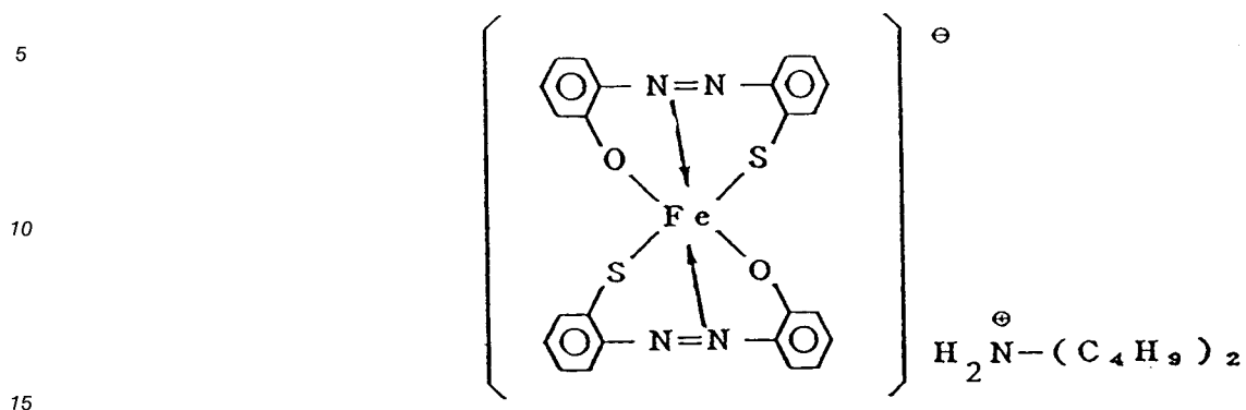
Complex [I]-5
