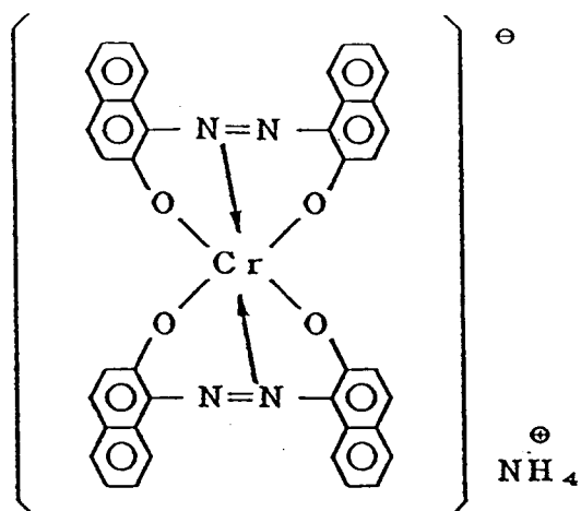
Complex [I]-1
