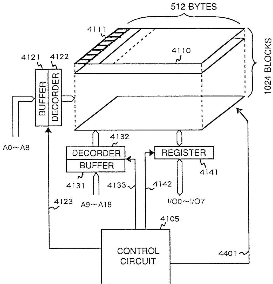
FIG. 97 PRIOR ART
