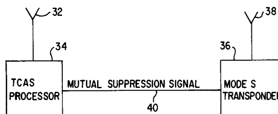
TCAS/MODE S MUTUAL SUPPRESSION SYSTEM
