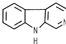
norharman
