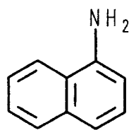
\alpha -naphthylamine
