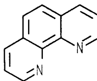
1,10-phenanthroline
