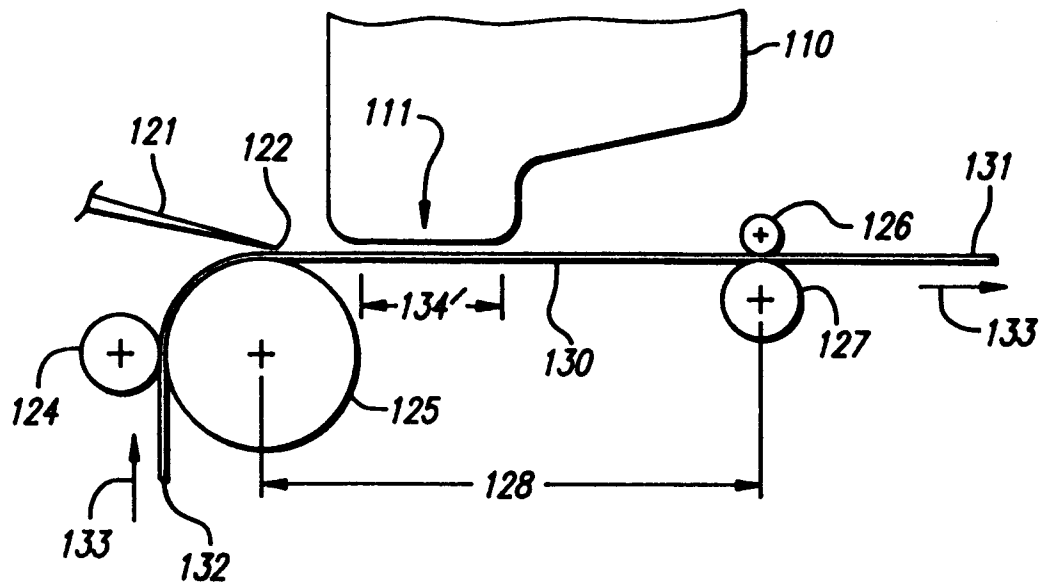
FIG. 4 PRIOR ART
