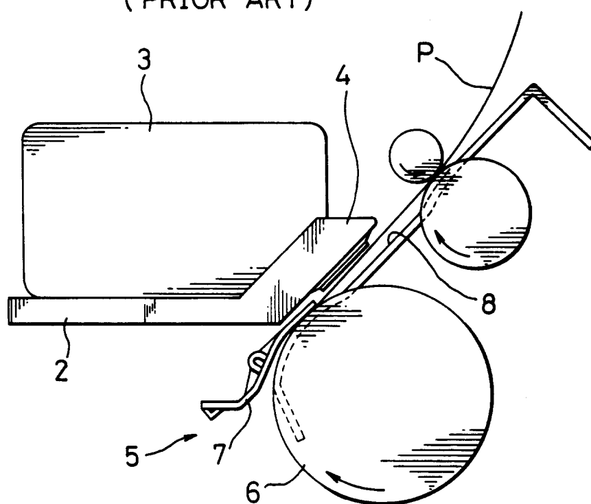
FIG.10 (PRIOR ART)
