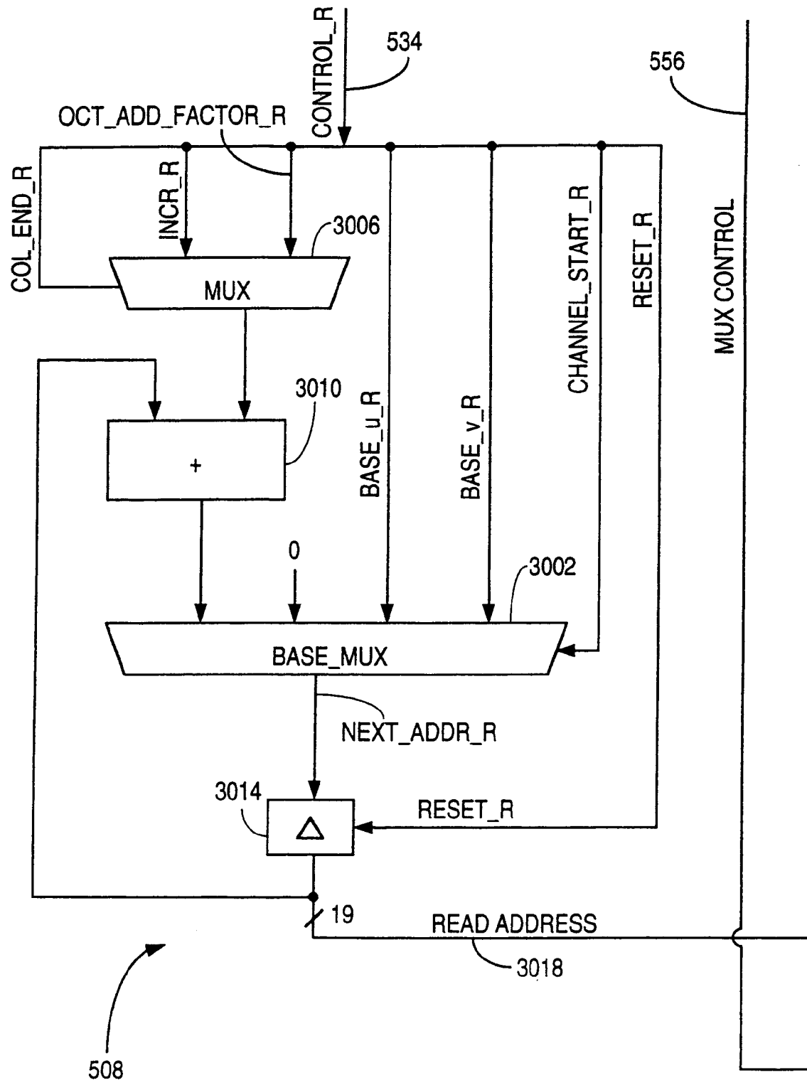
FIG. 30A DWT ADDRESS GENERATOR
