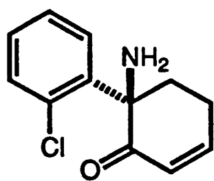
( R )-5,6-DNK
