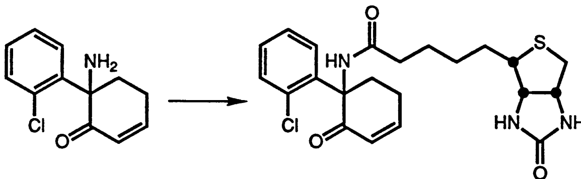
6-Biotinoylamino-6-(2-chlorophenyl)-2-cyclohexen-1-one
