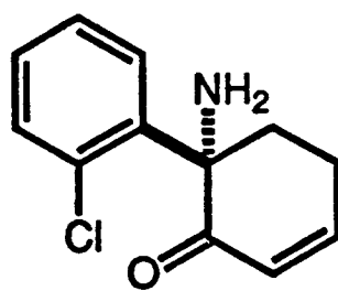
( S )-5,6-DNK
