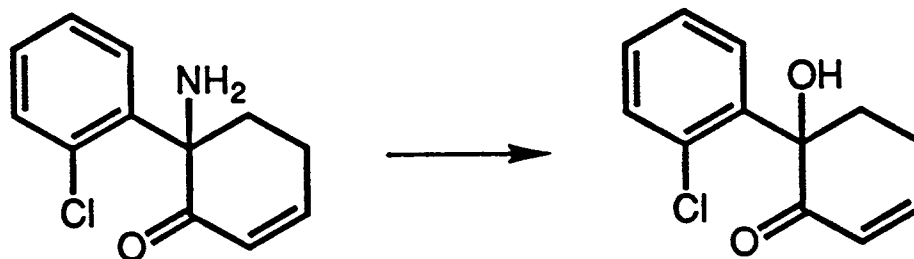
6-(2-Chlorophenyl)-6-hydroxy-2-cyclohexen-1-one
