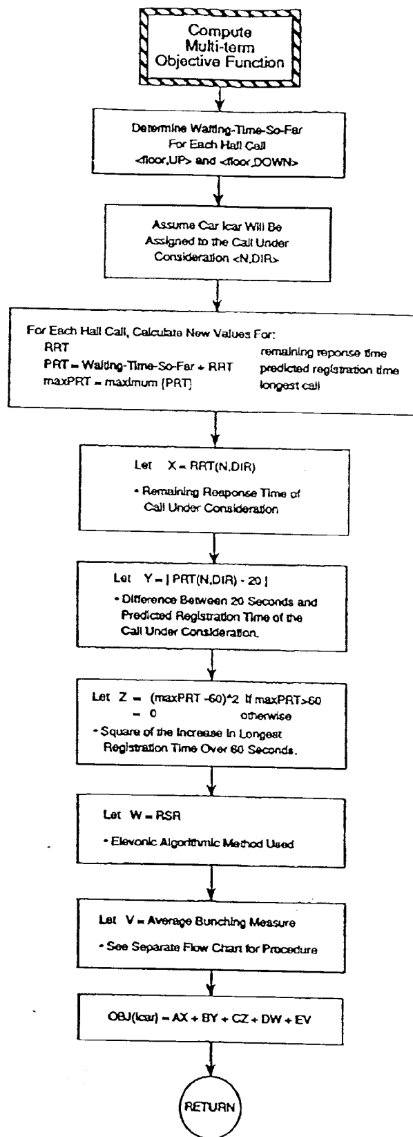
Figure 19. Multiple Term Objective Function
