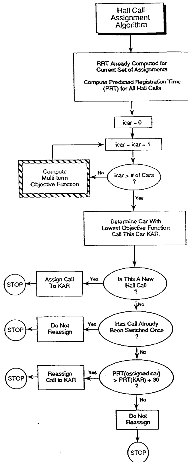
Figure 18. Hall Call Assignment Algorithm
