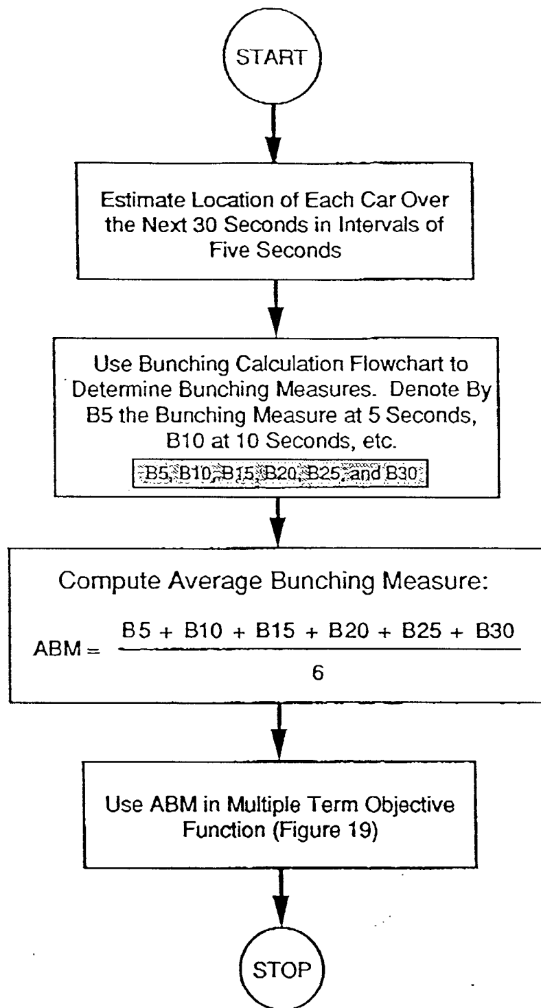
Figure 16. Calculate Average Bunching Measure Over Next 30 Seconds
