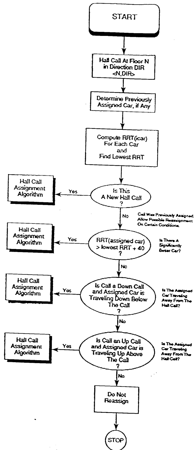
Figure 17. Master Flow Chart
