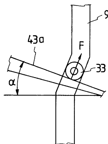
FIG. 13D
