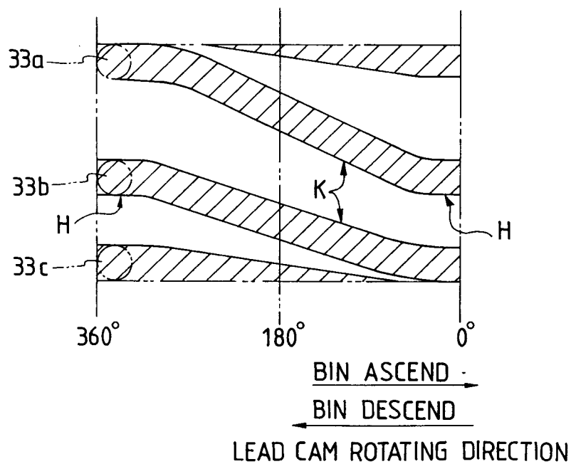
FIG. 3 PRIOR ART
