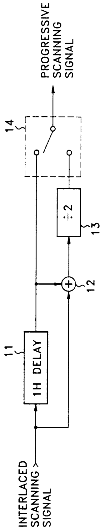
FIG. 1 (PRIOR ART)
