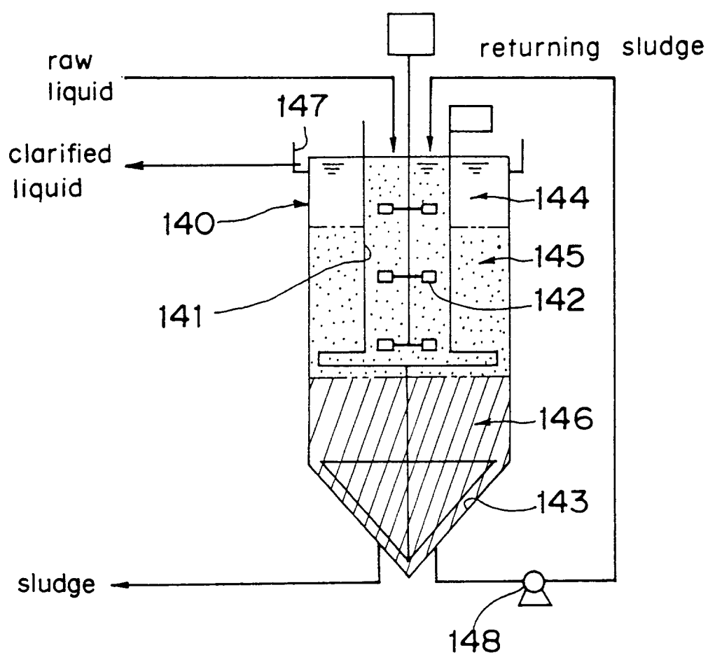
Fig. 8 PRIOR ART
