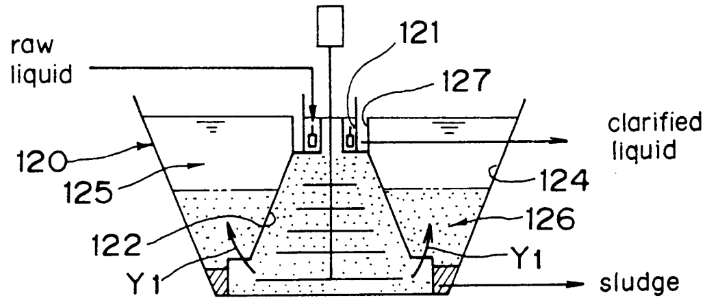
Fig. 6 PRIOR ART
