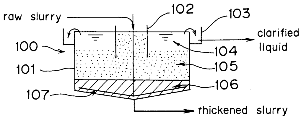
Fig. 4 PRIOR ART
