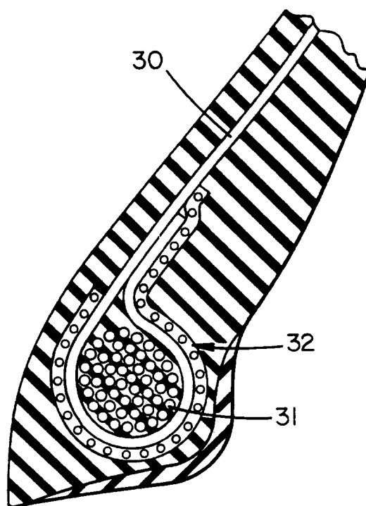
FIG. 3 (PRIOR ART)
