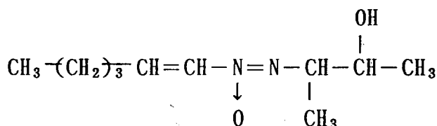
KA-7367B (Maniwamycin B)
