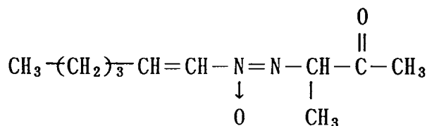
KA-7367A (Maniwamycin A)
