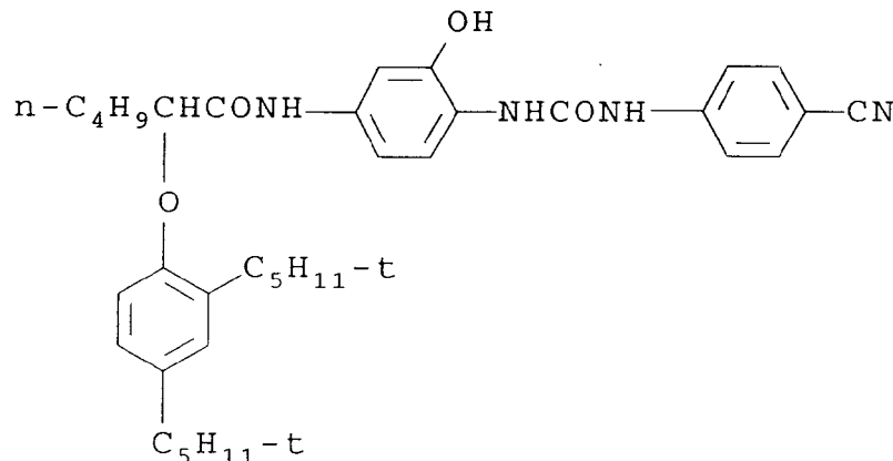
Coupler C4
