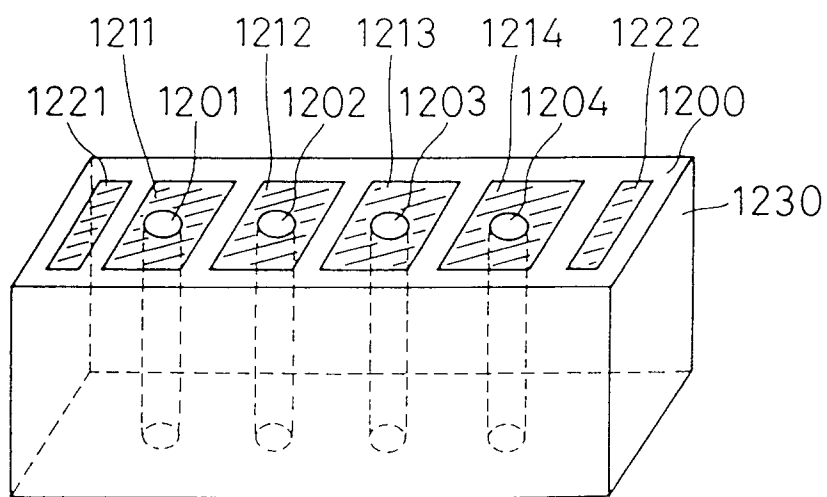
(PRIOR ART) FIG. 47
