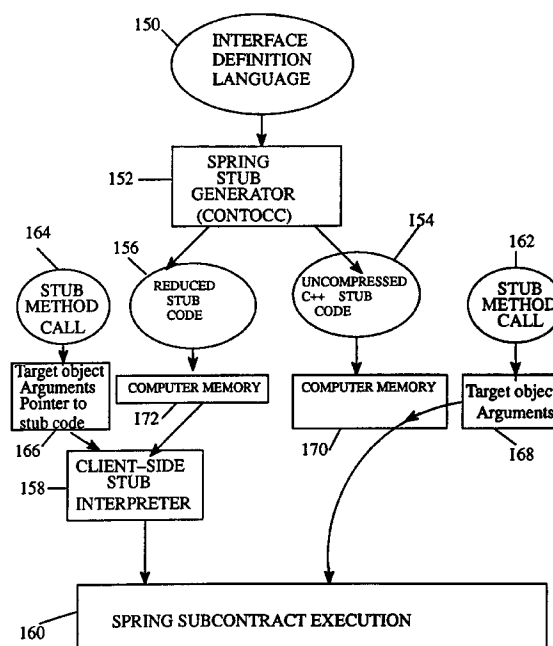
CLIENT-SIDE STUB INTERPRETER COMPONENTS FIG. 2
