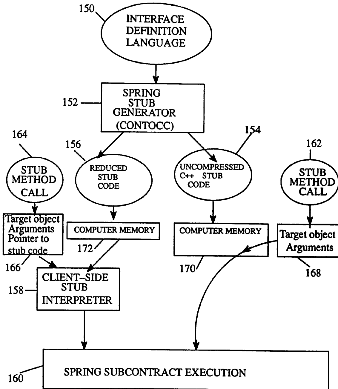
CLIENT-SIDE STUB INTERPRETER COMPONENTS
