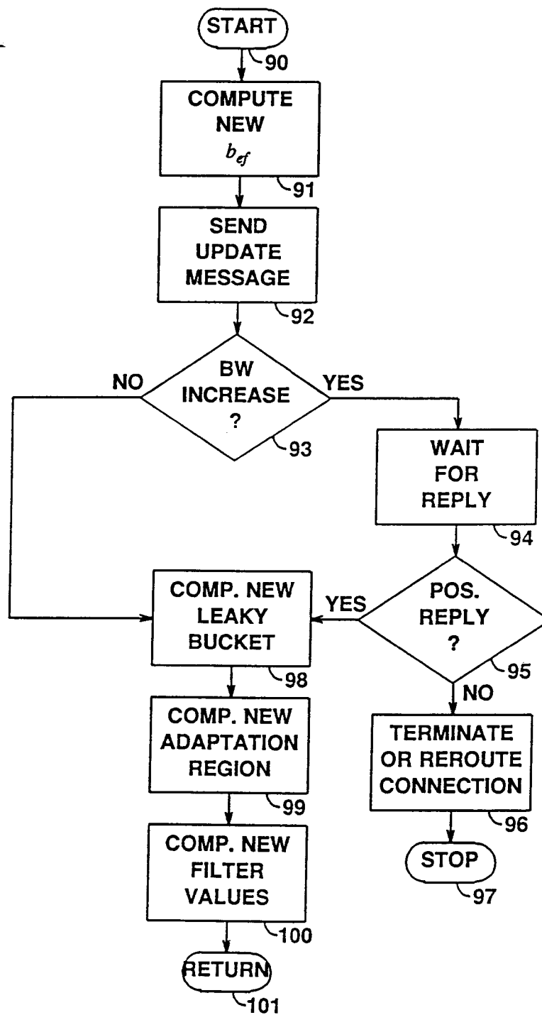
FIG. 8 UPDATING CONNECTION
