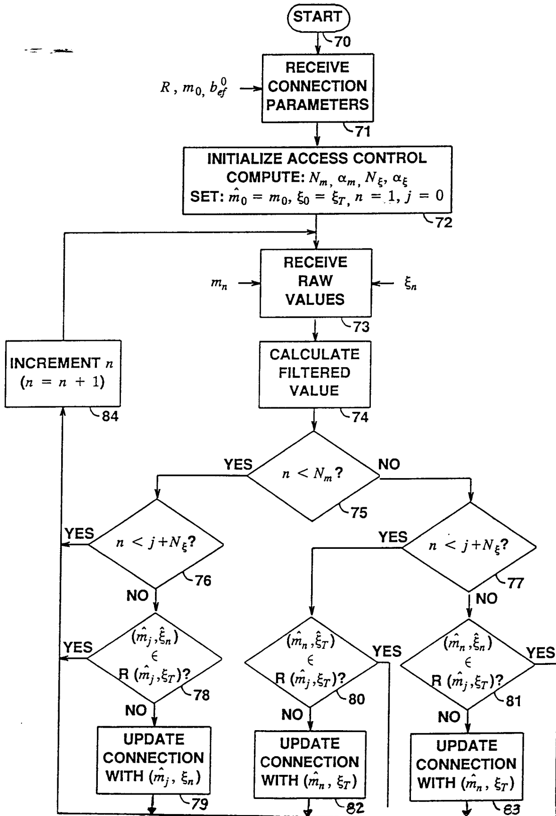
FIG. 7 ACCESS CONTROL FLOW CHART
