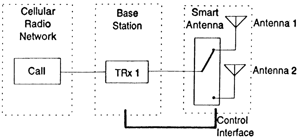
Fig. 4 (b) Cellular System with Smart Antenna
