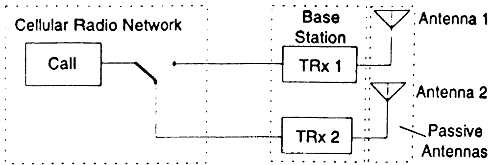
Fig. 4 (a) Conventional Cellular System
