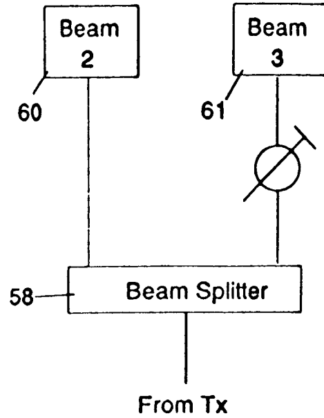
Fig. 14 (b) Quadrature
