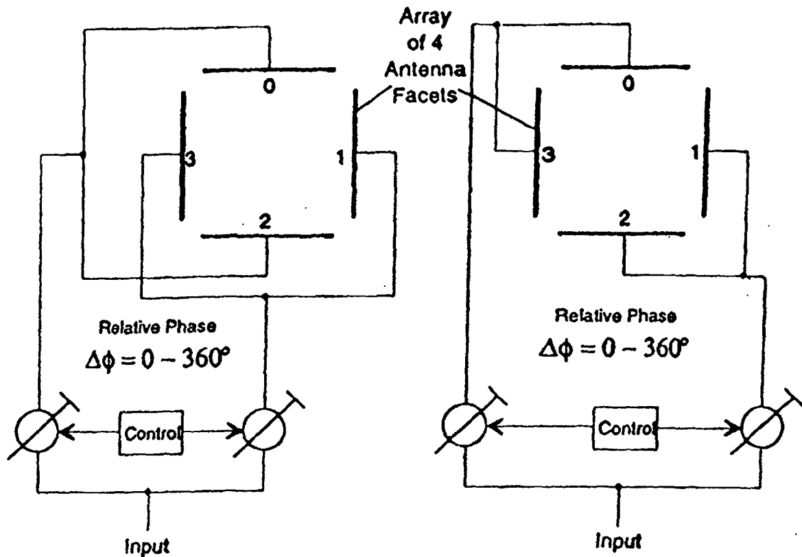
Fig.12 (b) Alternative Embodiment
