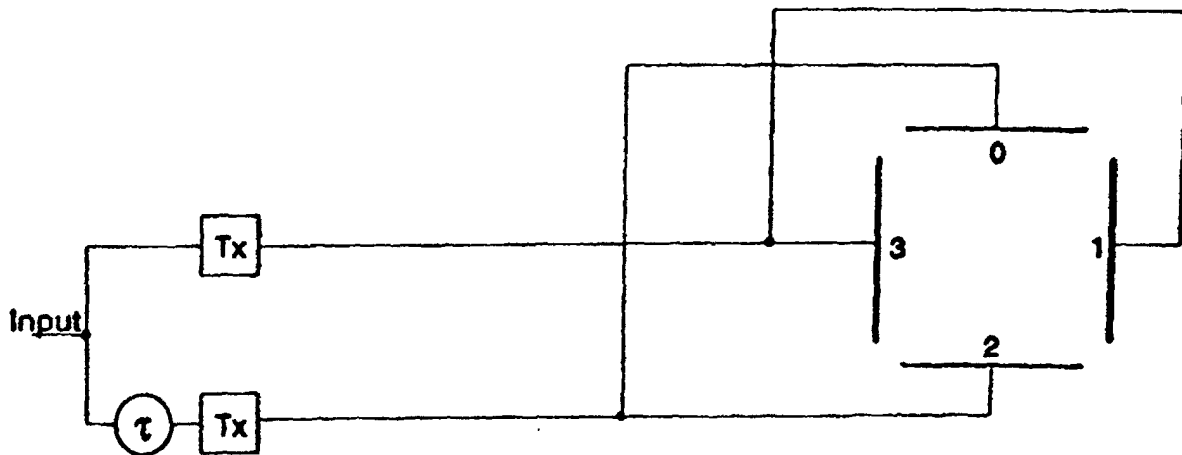
Fig. 12 (c) Transmit Diversity Embodiment
