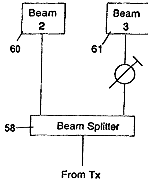
Fig. 14 (b) Quadrature
