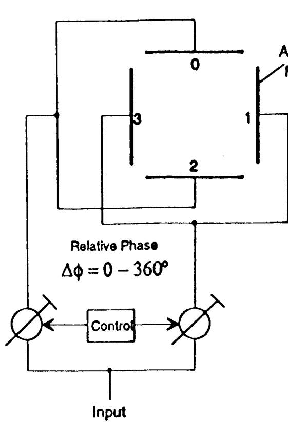
Fig. 12 (a) Preferred Embodiment
