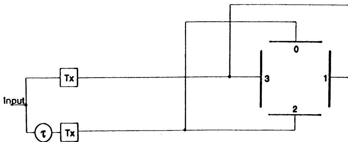
Fig. 12 (c) Transmit Diversity Embodiment
