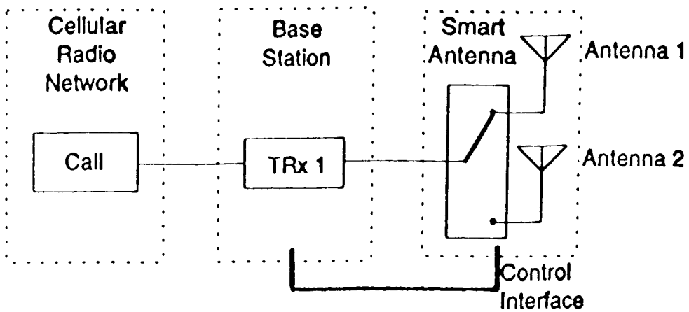
Fig. 4 (b) Cellular System with Smart Antenna
