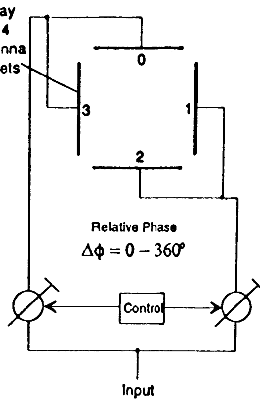
Fig.12 (b) Alternative Embodiment
