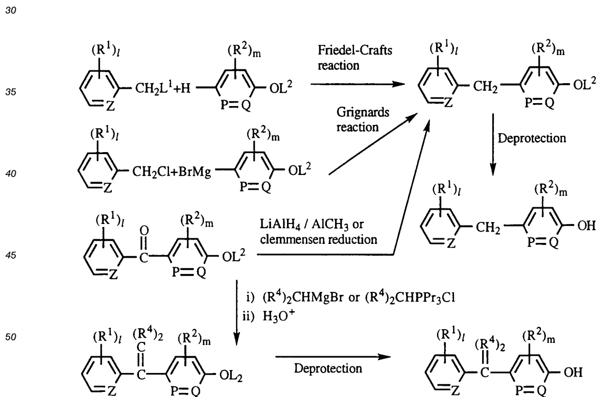
Scheme 3. The symbols are the same as defined above.
