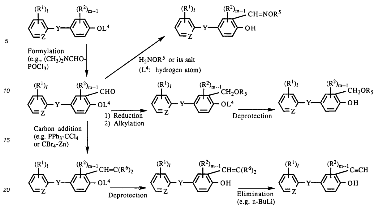
Scheme 8. \text{L}^4 is a hydrogen or methoxymethyl; \text{R}^5 is an alkyl of \text{C}_1\text{-C}_3 ; \text{R}^6 is chlorine or bromine; and other symbols are the same as defined above.
