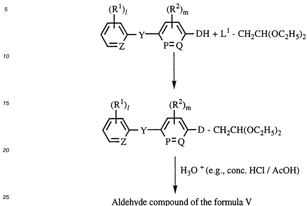
Scheme 10. The symbols are the same as defined above.
