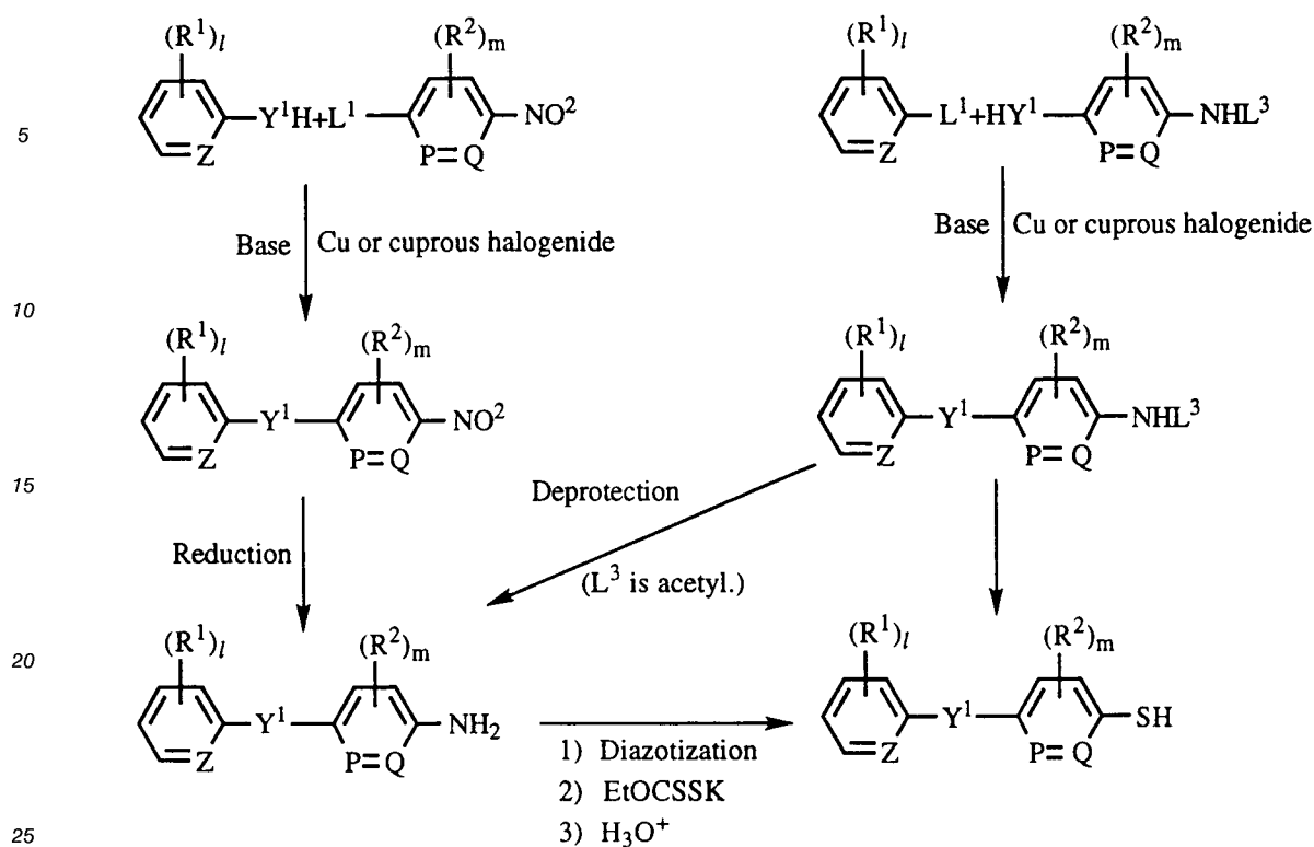
Scheme 2. L^3 is hydrogen or acetyl; and other symbols are the same as defined above.
