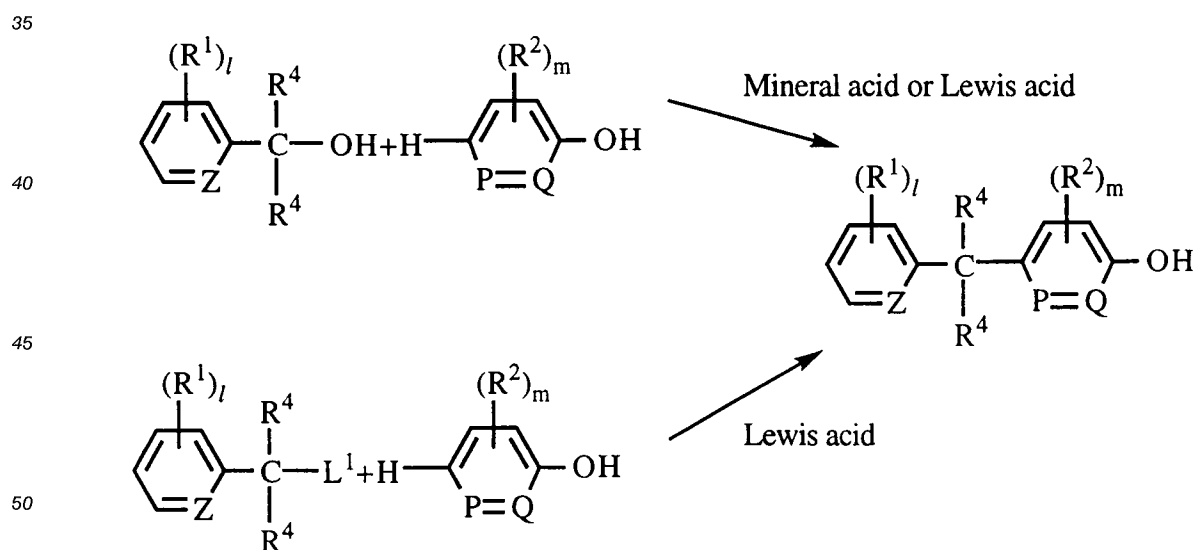
Scheme 5. The symbols are the same as defined above.
