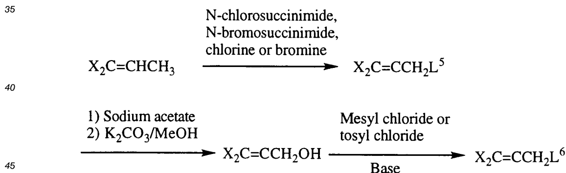
Scheme 11. L^5 is chlorine or bromine, L^6 is mesyloxy or tosyloxy, and X is the same as defined above.
