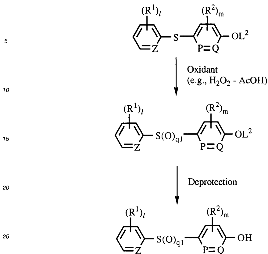
Scheme 4. q^1 is an iterger of 1 or 2, and other symbols are the same as above.
