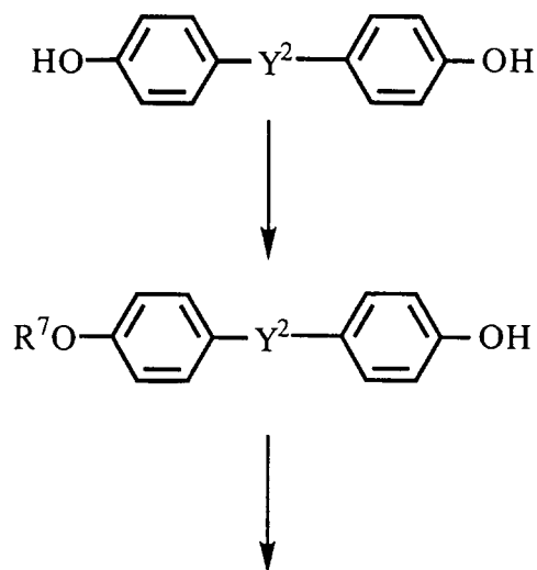
Compounds shown in Scheme 6 and 7
