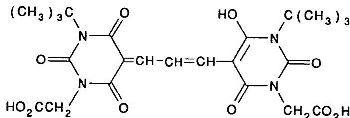
Dye A: bis-[1-butyl-3-carboxymethylbarbituric acid-(5)]trimethineoxonol.
