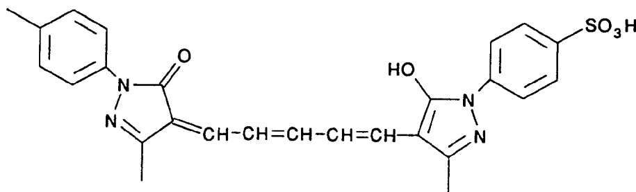
Dye B: bis-[3-methyl-1-p-sulphophenyl-5-pyrazolone-(4)]pentamethineoxonol.
