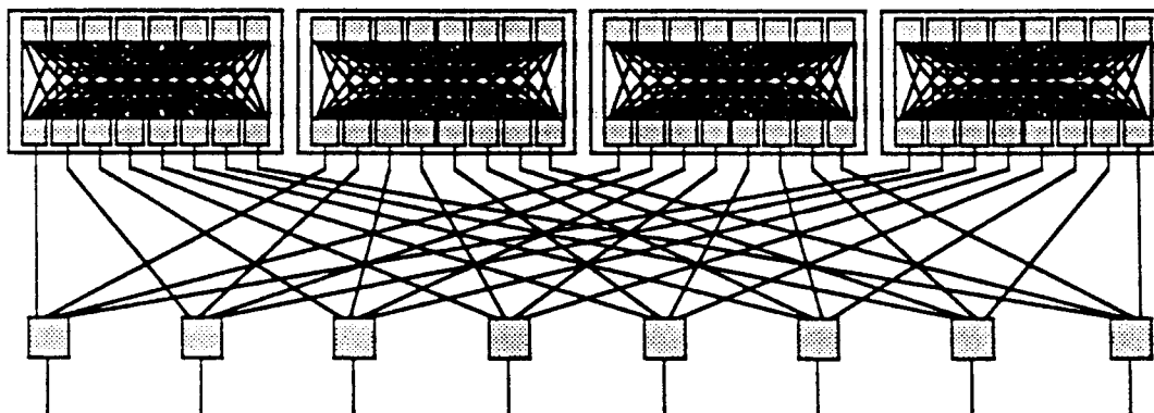
CONNECTIONS TO OTHER CARDCAGES
