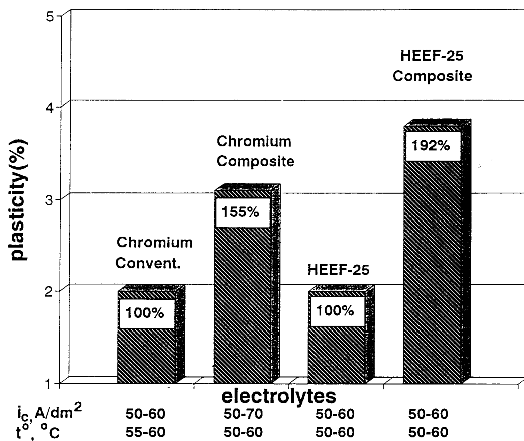
Fig.3 Plasticity comparison of chromium coatings deposited from electrolytes according to the present invention and known electrolytes
