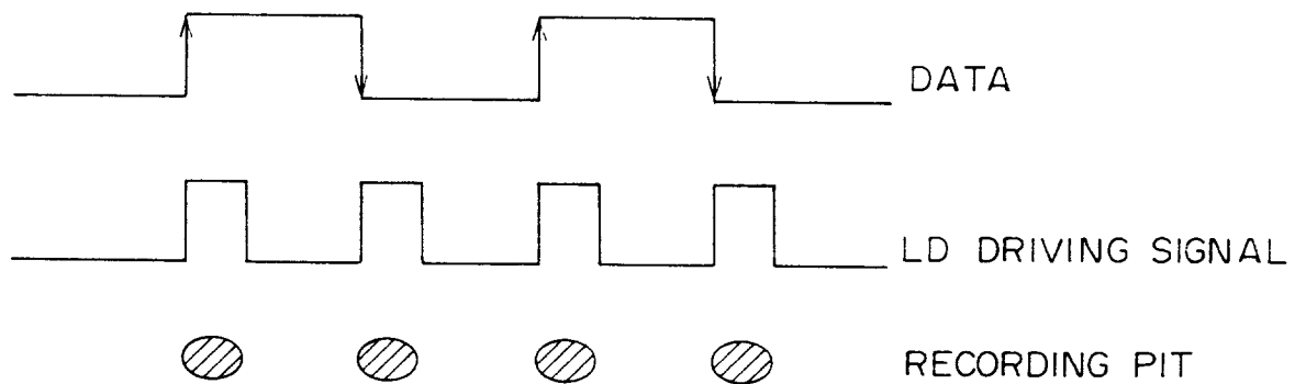
FIG. 2 (PRIOR ART)
