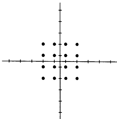
CONSTELLATION C FOUR BITS PER SYMBOL 9600 bps
