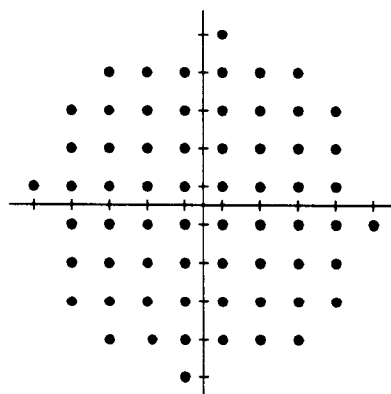
CONSTELLATION E SIX BITS PER SYMBOL 14400 bps
