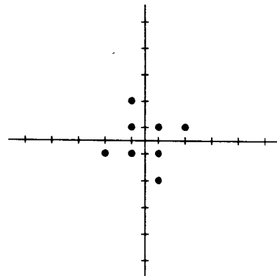
CONSTELLATION B THREE BITS PER SYMBOL 7200 bps
