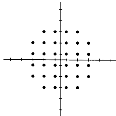
CONSTELLATION D FIVE BITS PER SYMBOL 12000 bps
