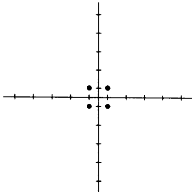
CONSTELLATION A TWO BITS PER SYMBOL 4800 bps
