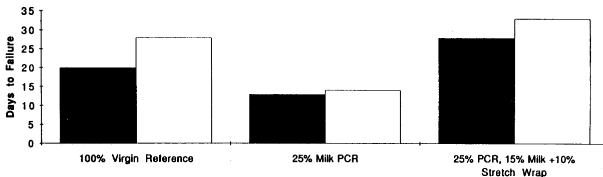
Fig. 1 Envionrmental Stress Crack Resistance 32 oz. Nonhandle, Square Base
