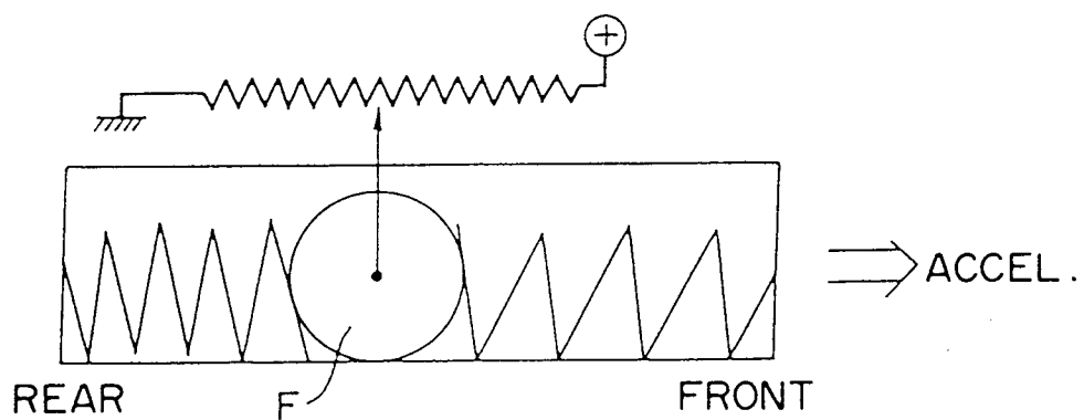
Fig. 16 PRIOR ART
