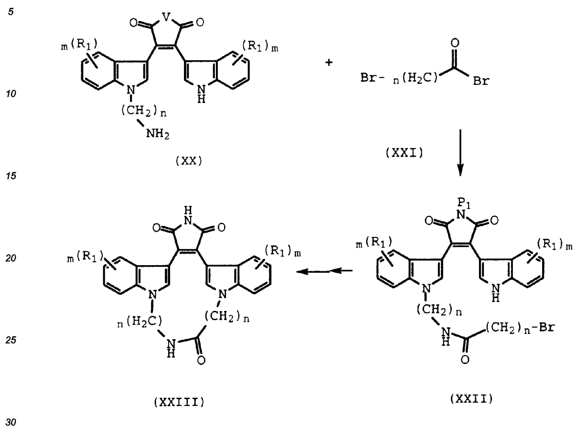
Scheme 6
