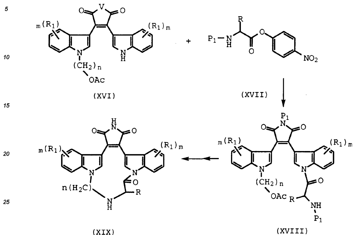
Scheme 5
