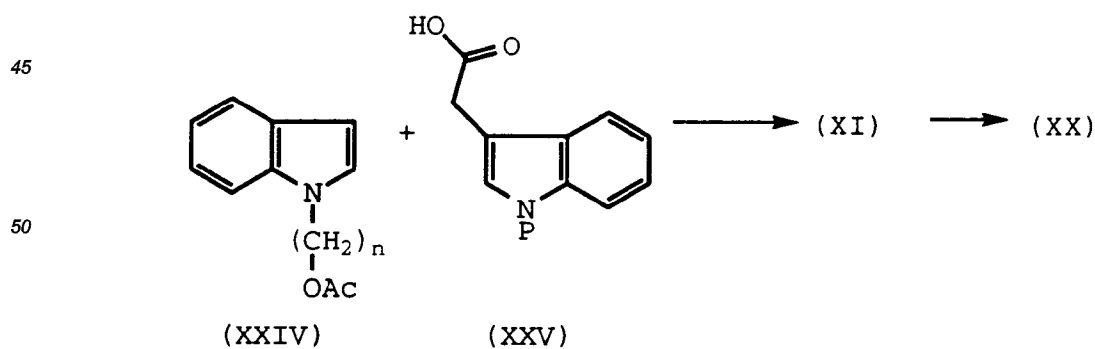
Scheme 7
