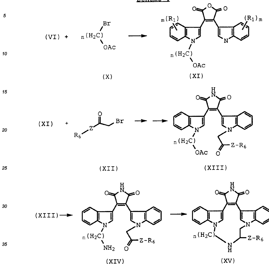
Scheme 4
