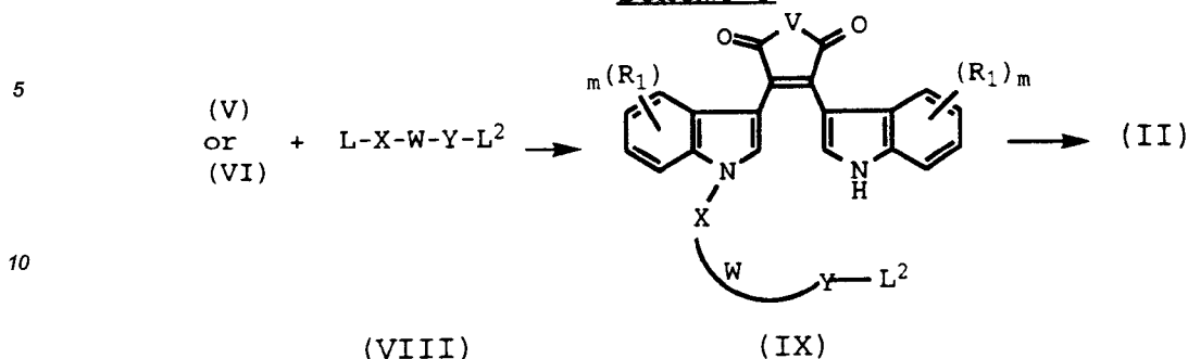
Scheme 3
