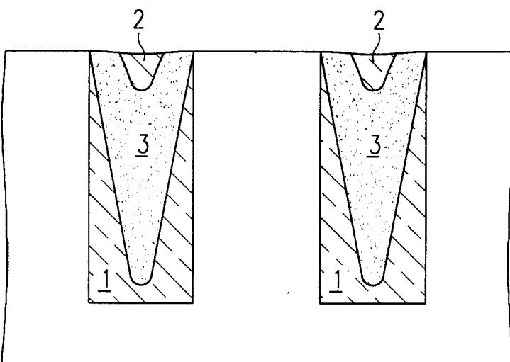
FIG. 3C SOG/LTO etchback
