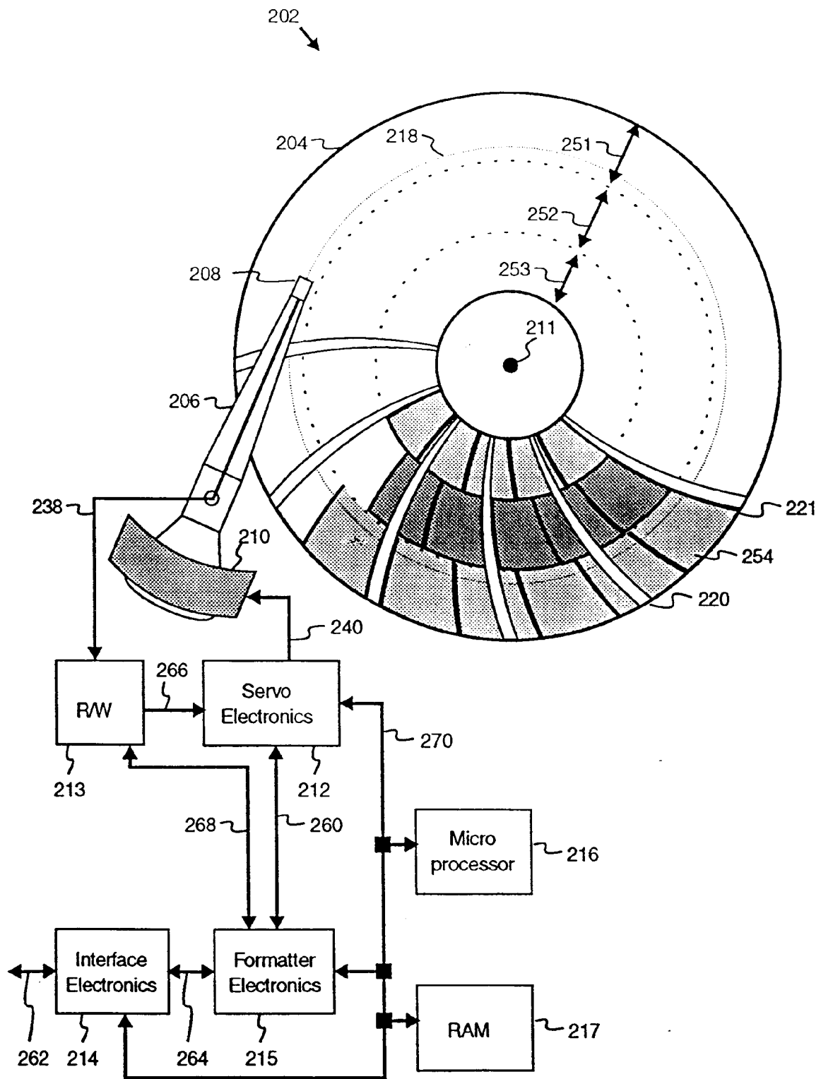
Disk Drive
