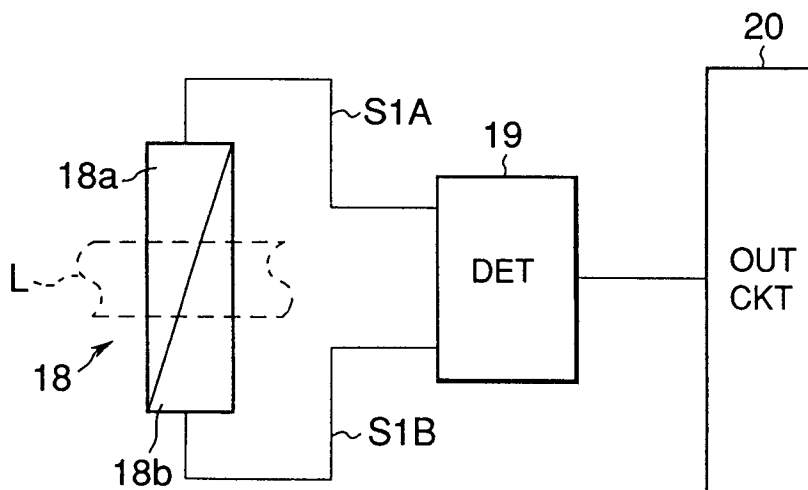
FIG. 13 PRIOR ART
